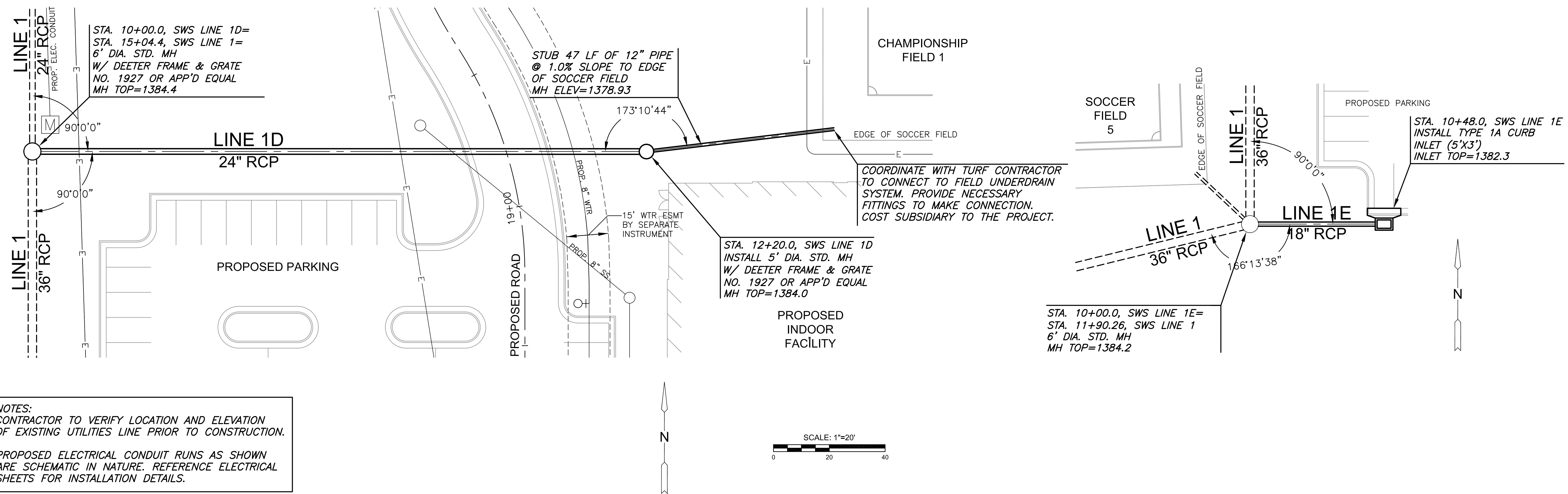
PLAN SWS LINE 1D PROFILE SWS LINE 1D
