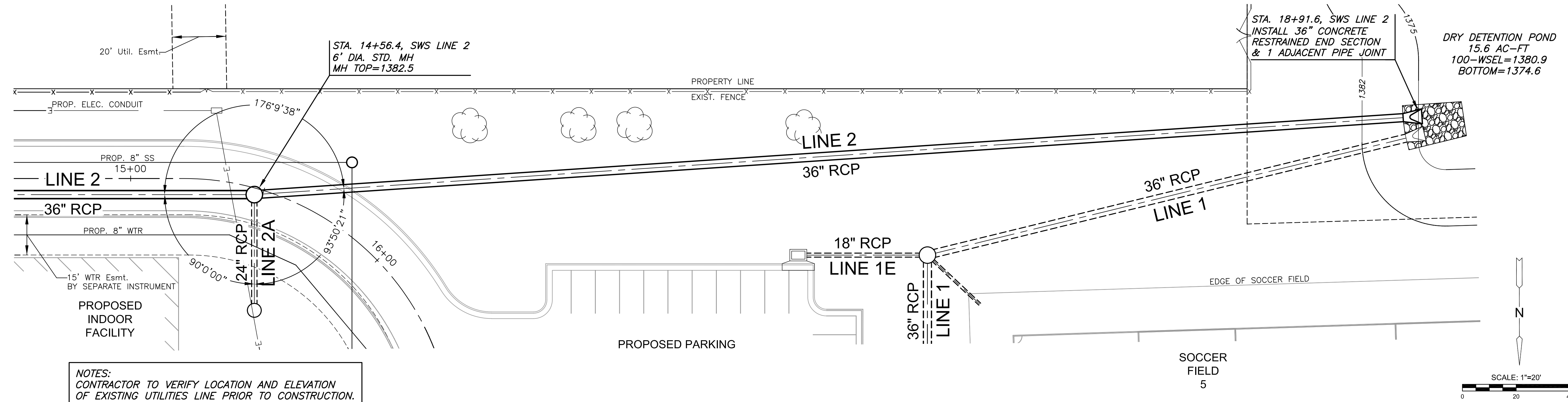
PLAN LINE 2 CONT. PROFILE LINE 2 CONT.
