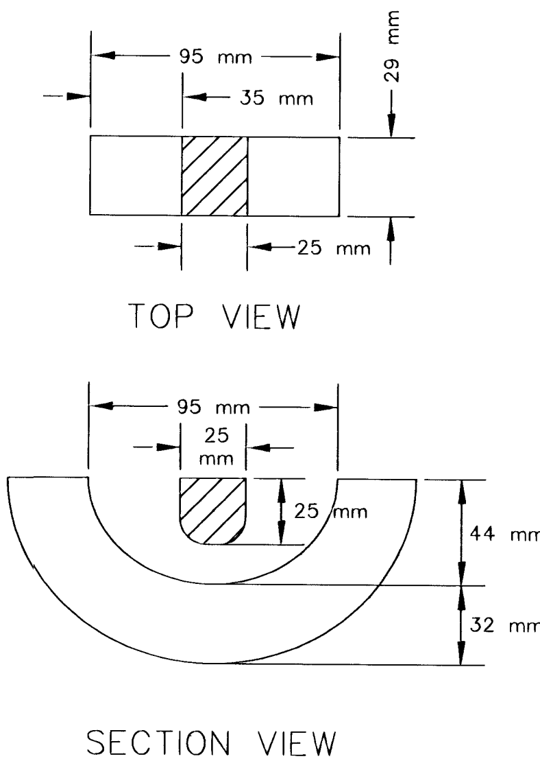
PICKHOLE DETAIL
