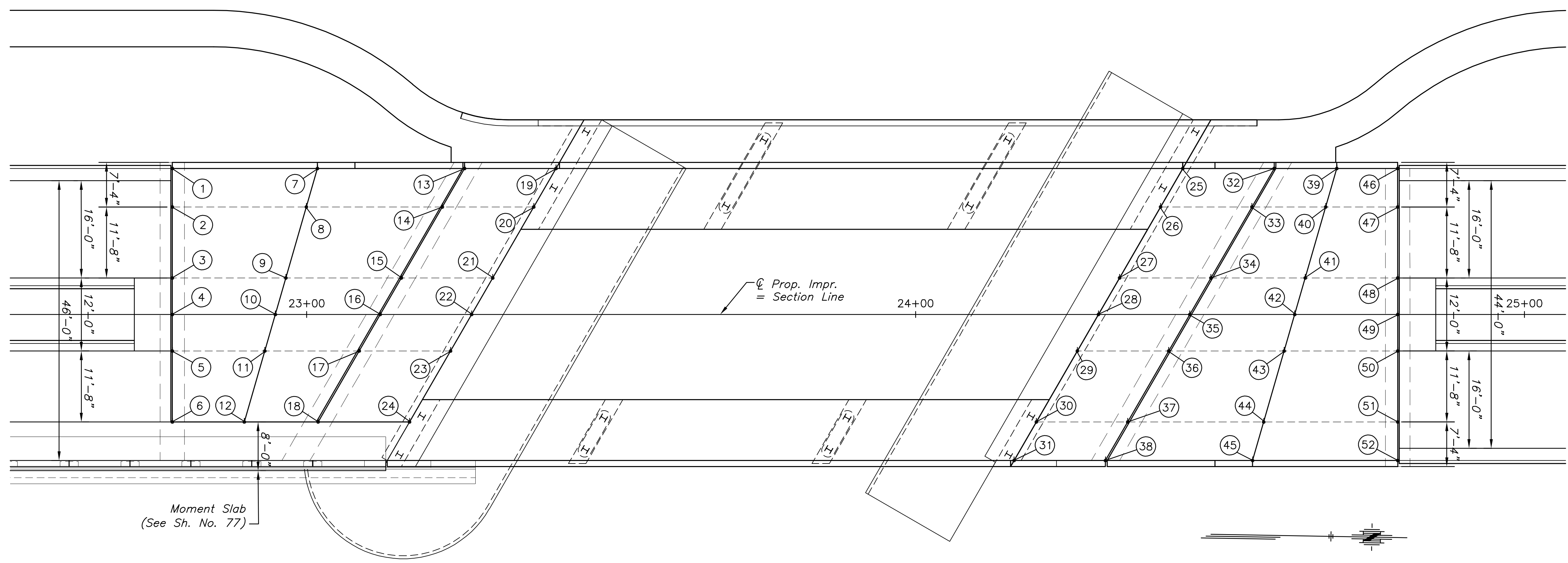
APPROACH SLAB ELEVATION PLAN
