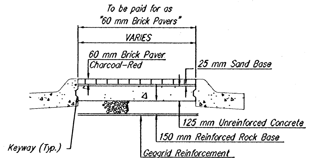
BRICK PAVER MEDIAN DETAIL
