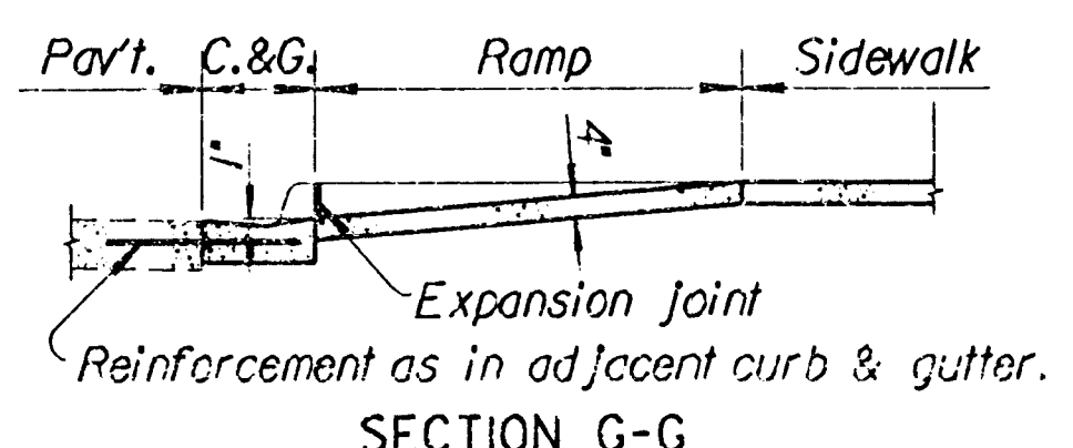
SECTION G-G
