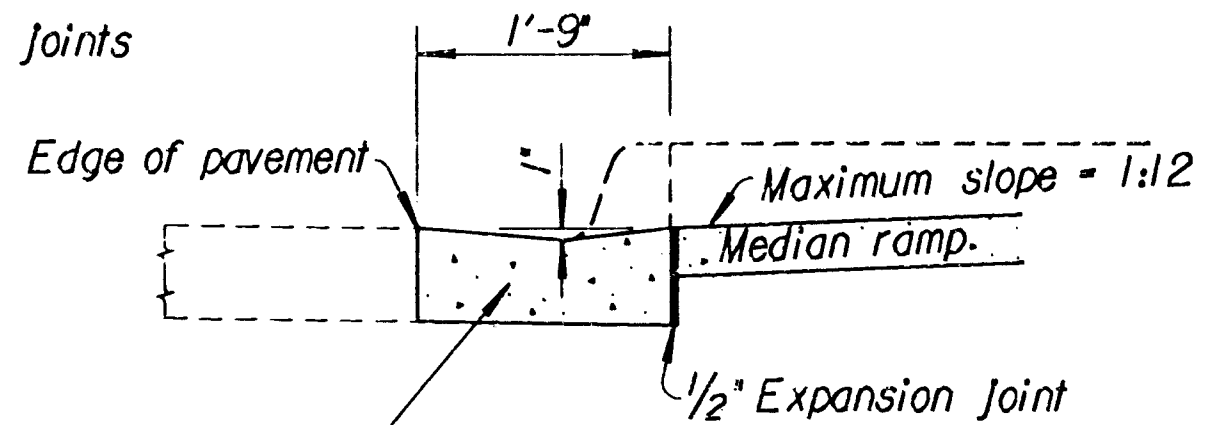
SECTION K-K
