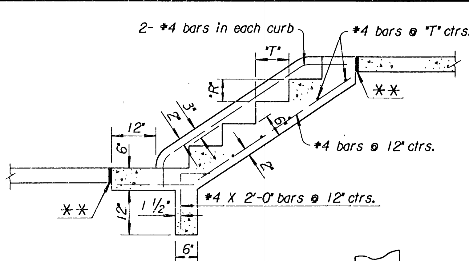
SECTION J-J
