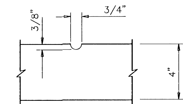
GROOVE DETAIL
