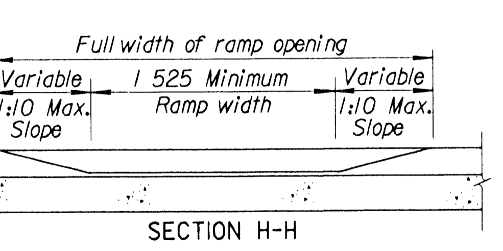
SECTION H-H
