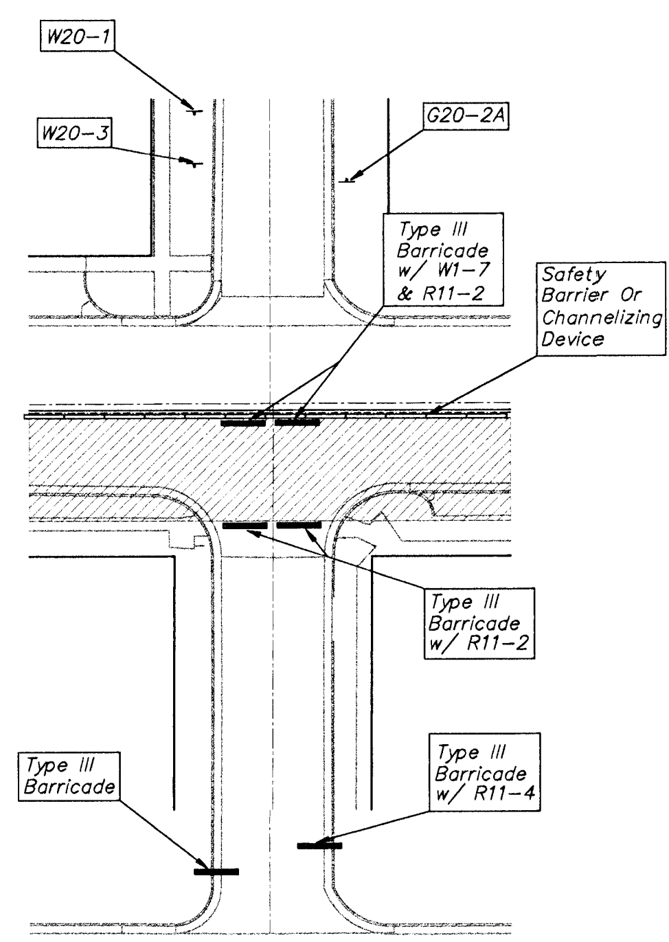
Typical Side Road Closed
