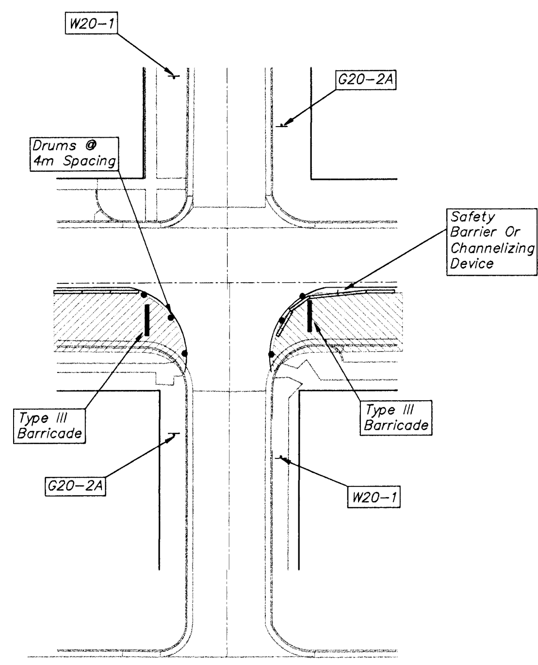
Typical Side Road Open
