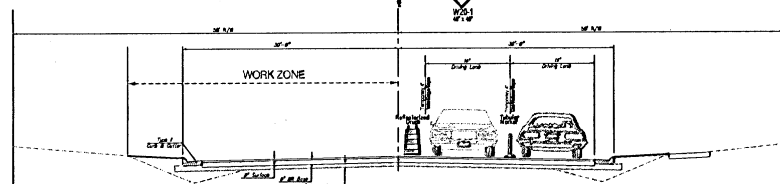
PHASE V (Looking North) Construct Roadway - West Side Hydraulic South of 57th Street to 50th Street Construct 7' A.C. Pavement on 8' Base
