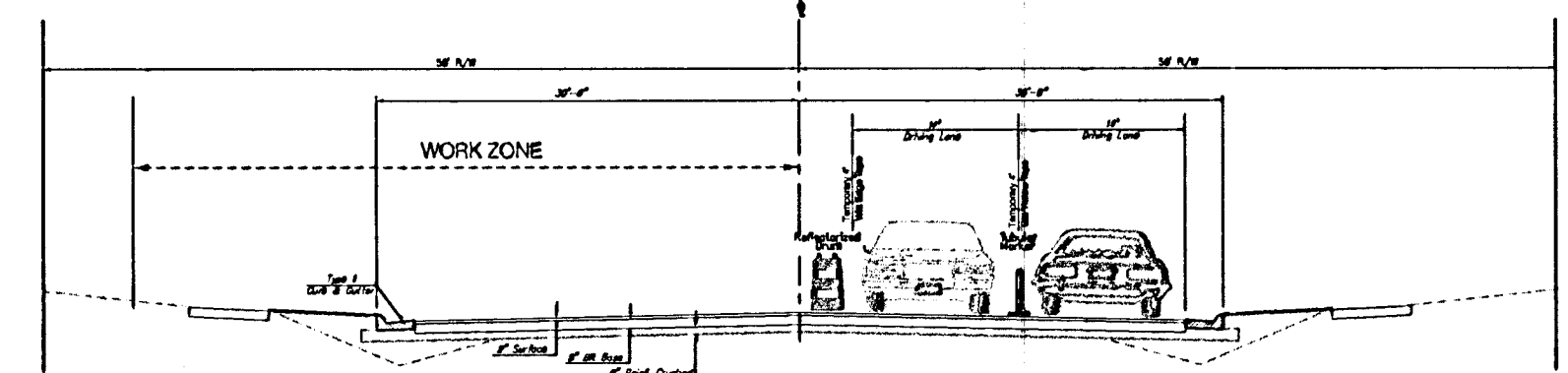
PHASE VI (Looking North) Continue Construction of Roadway - West Side Hydraulic South of 57th Street to 50th Street
