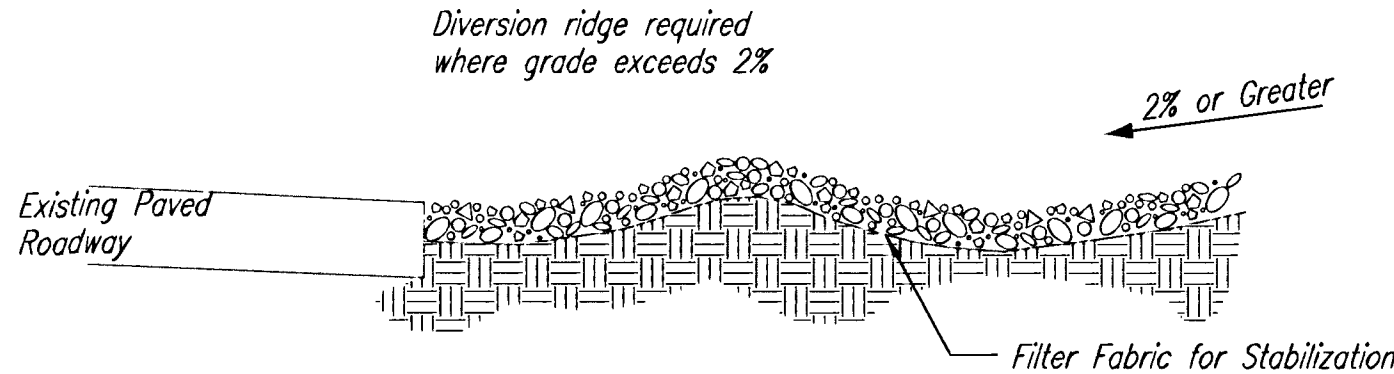
SECTION C-C
