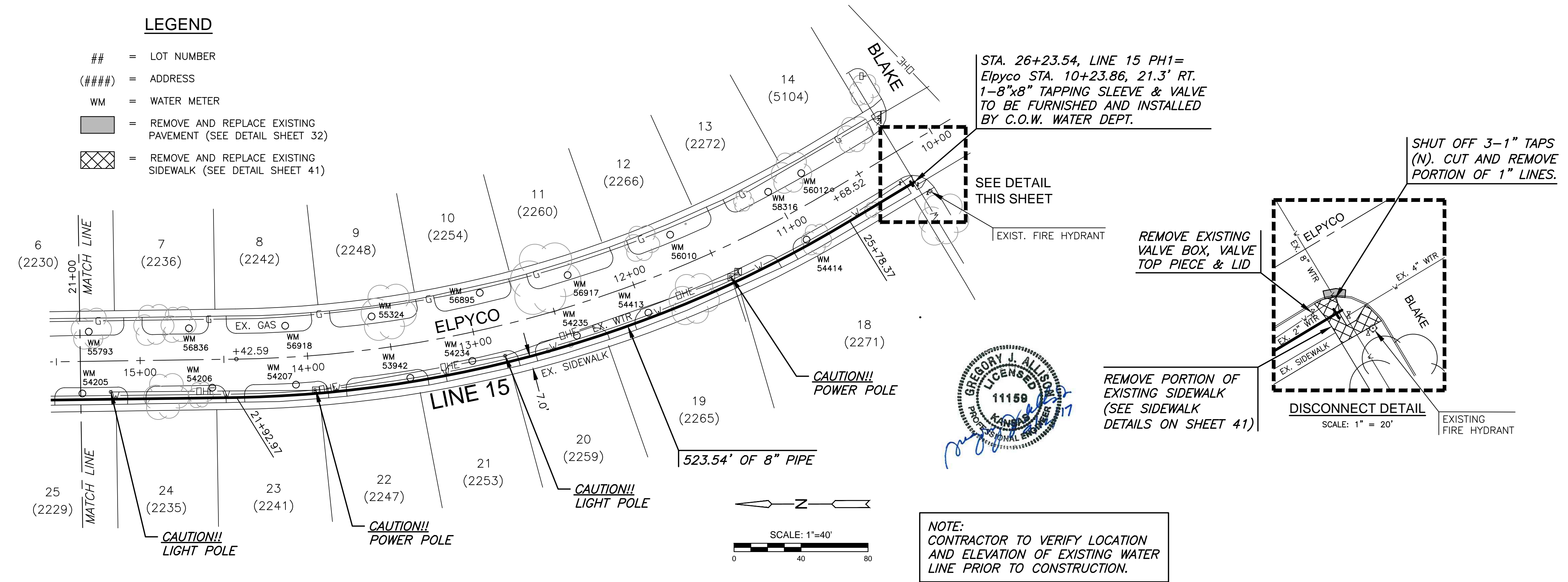
PLAN LINE 15 PH 1 (CONT.) PROFILE LINE 15 PH 1 (CONT.)
