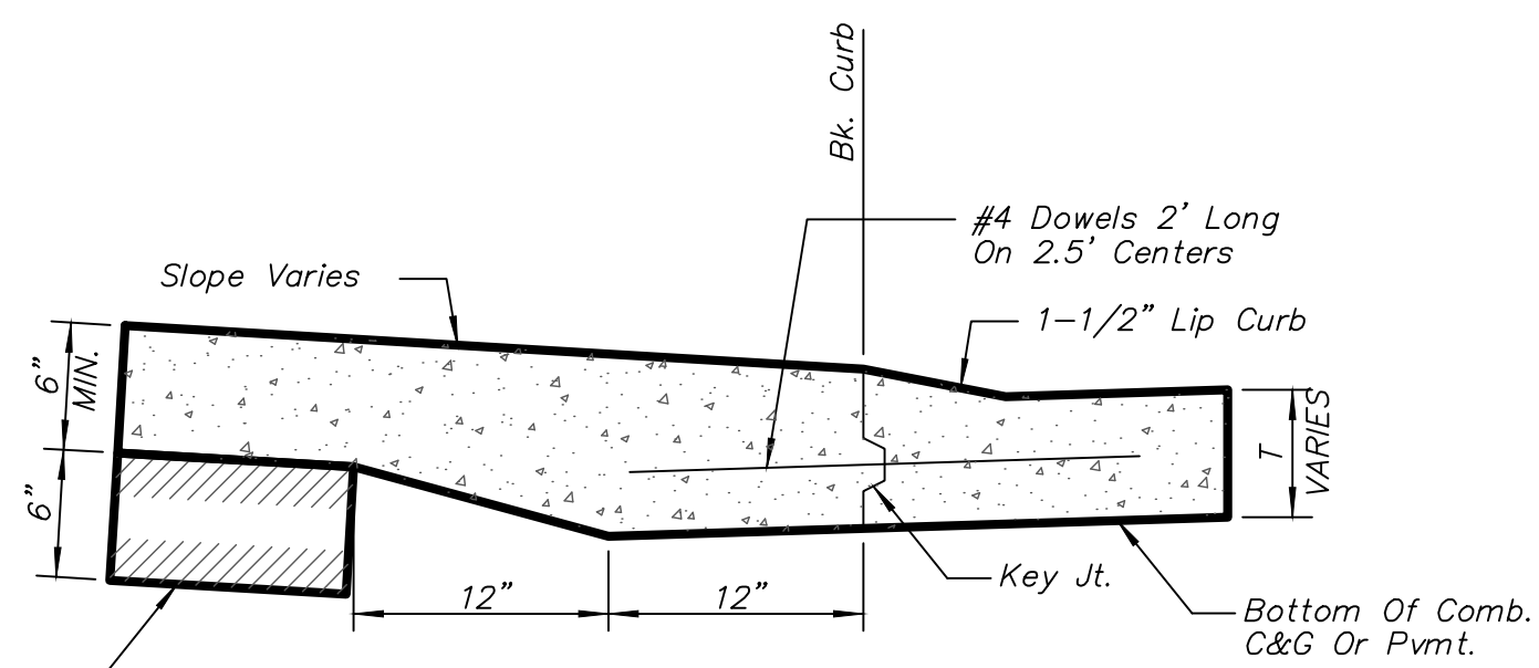
BACK OF CURB DETAIL
