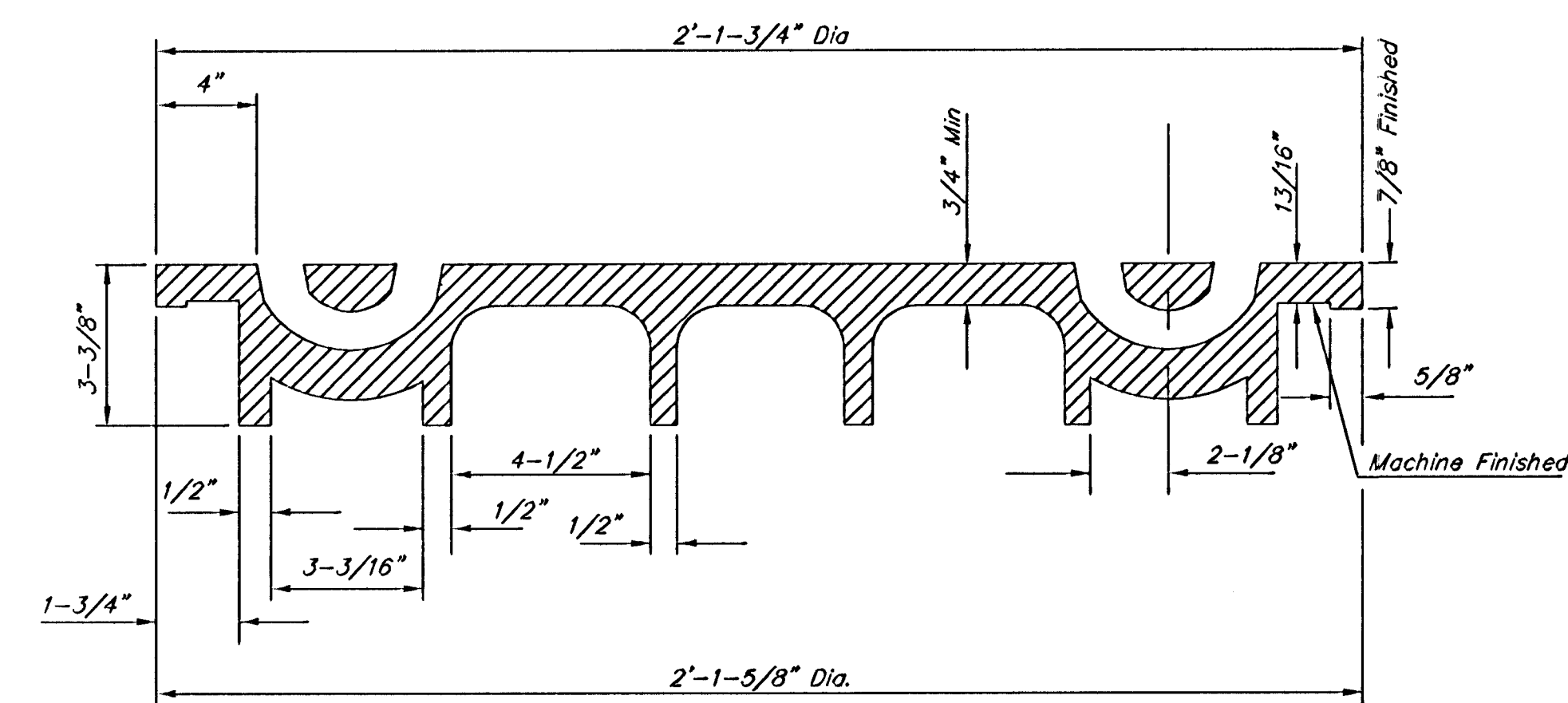
SECTION VIEW
