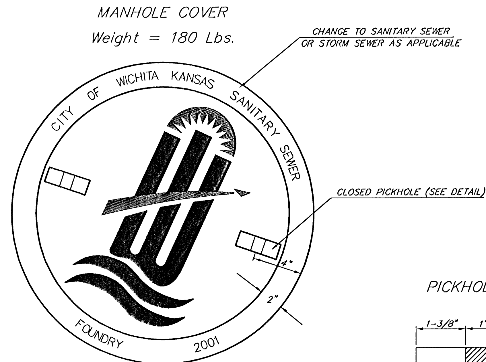
TOP VIEW
