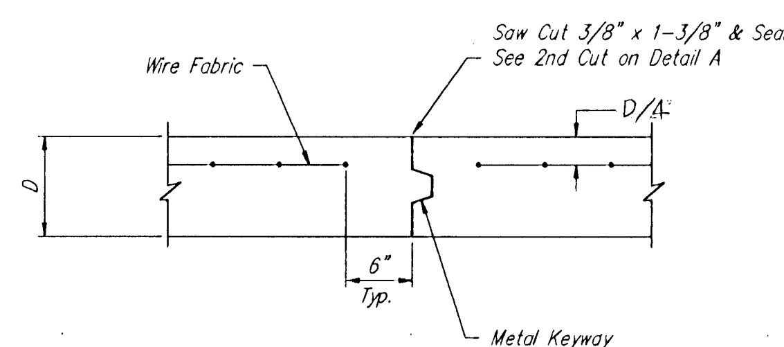
OPTIONAL CONTRACTION CONST. JOINT (C.J.) (ALTERNATE C.J.)
