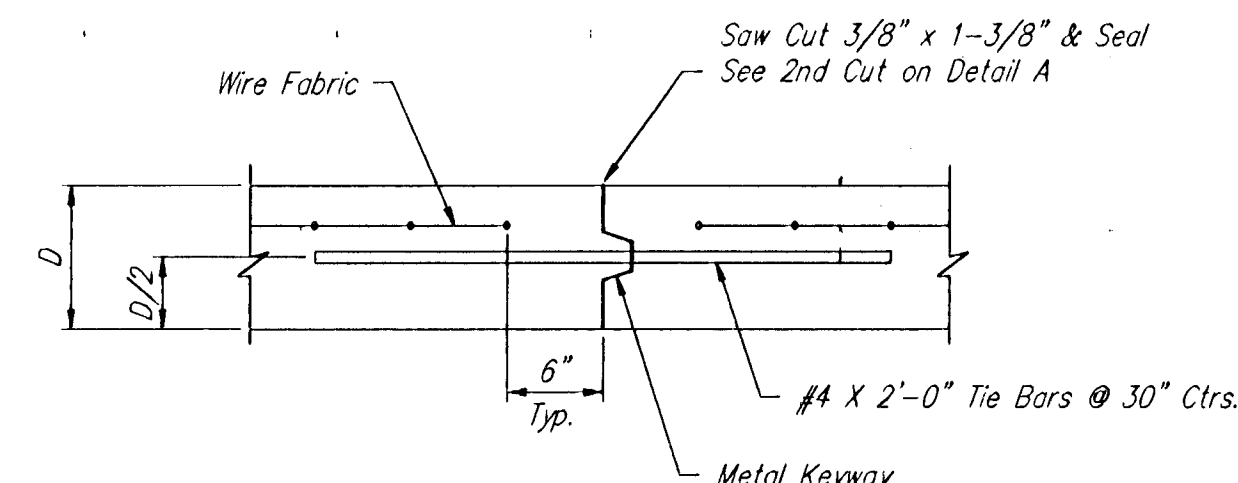
LONGITUDINAL JOINT DETAIL (L.J.)
