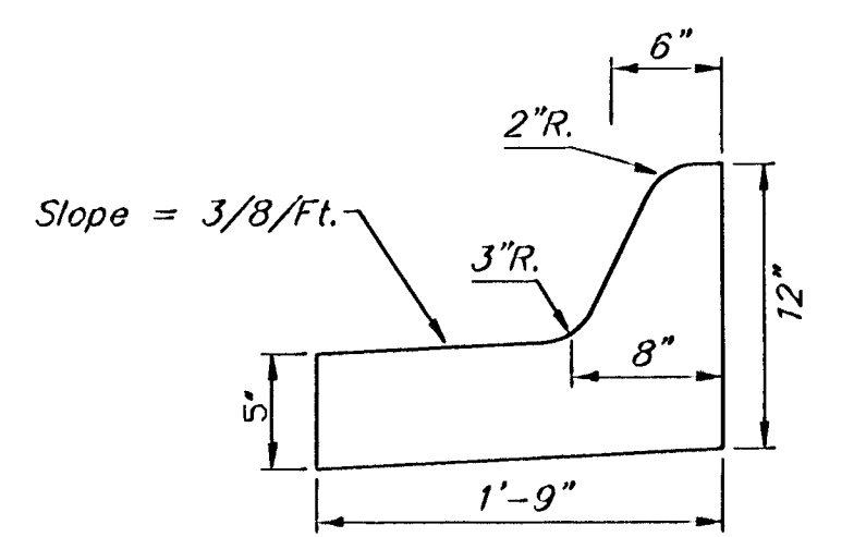
Median Curb Detail (Low Edge) Not to Scale
