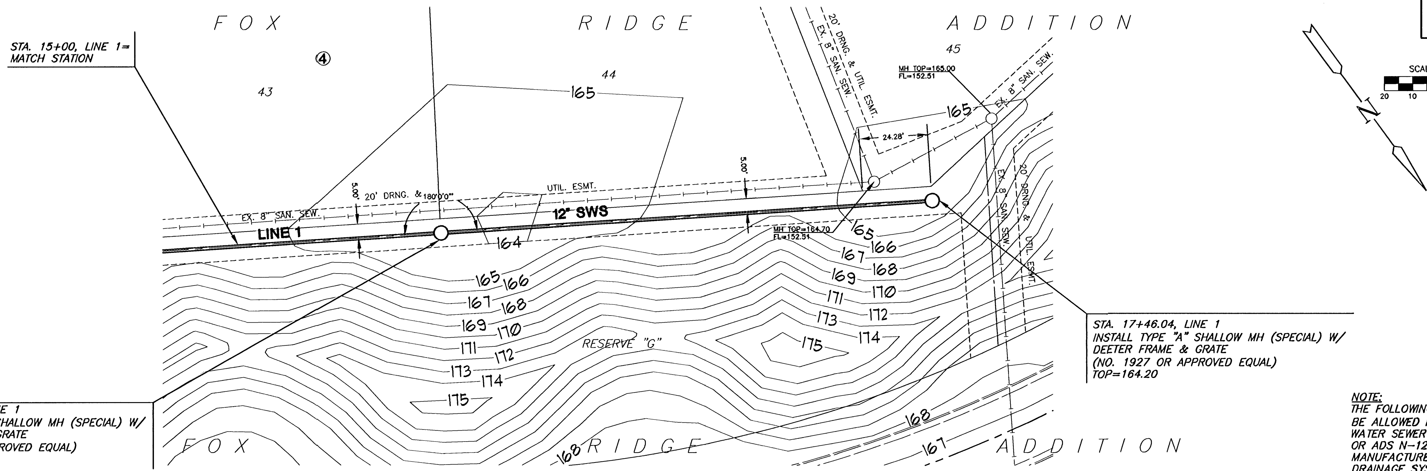
PLAN LINE 1 SCALE: 1"=20'
