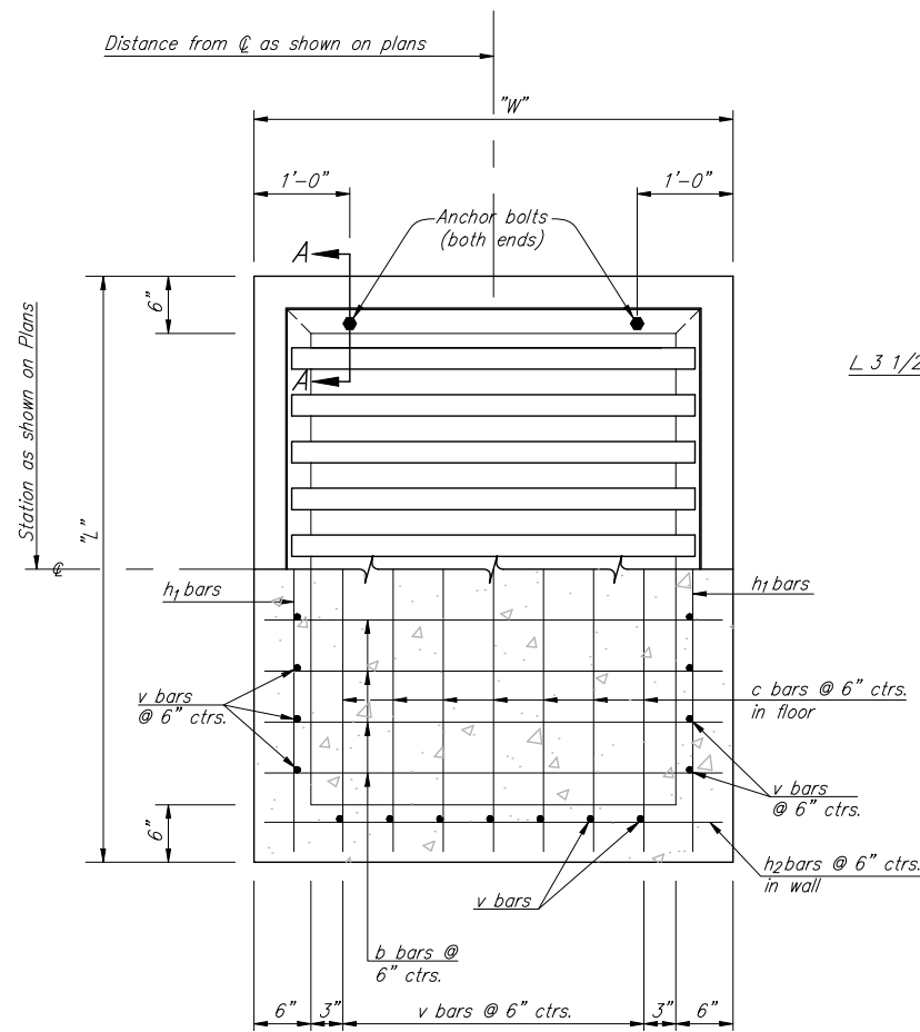
PLAN AND SECTION
