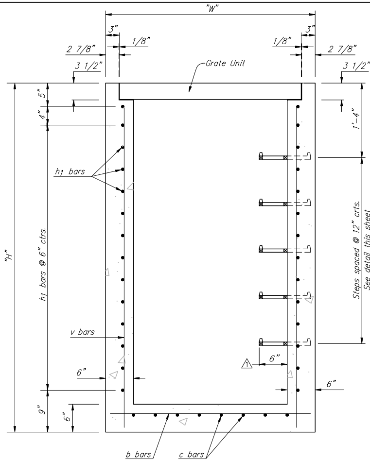
SECTION
