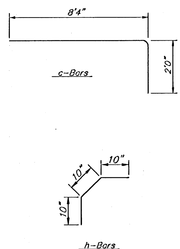
HEADWALL FOR 36" RCP
