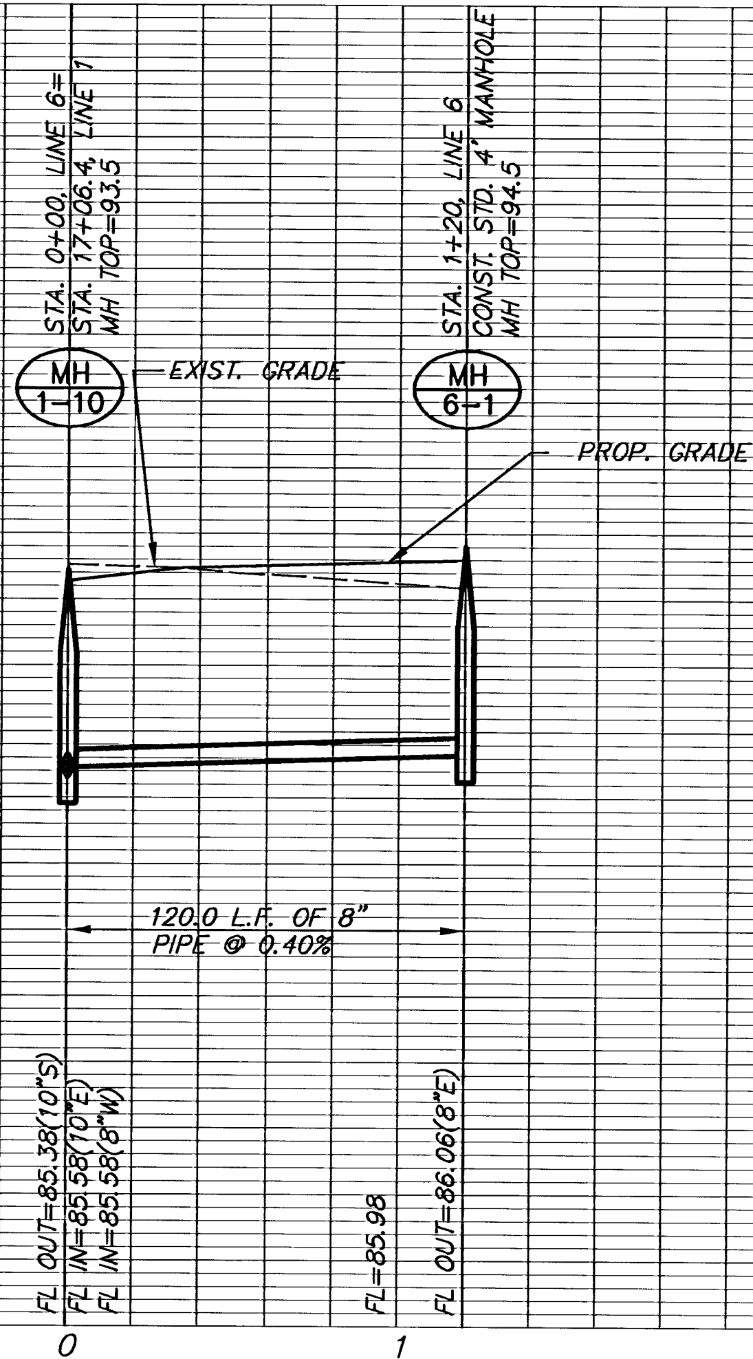
PROFILE LINE 6
