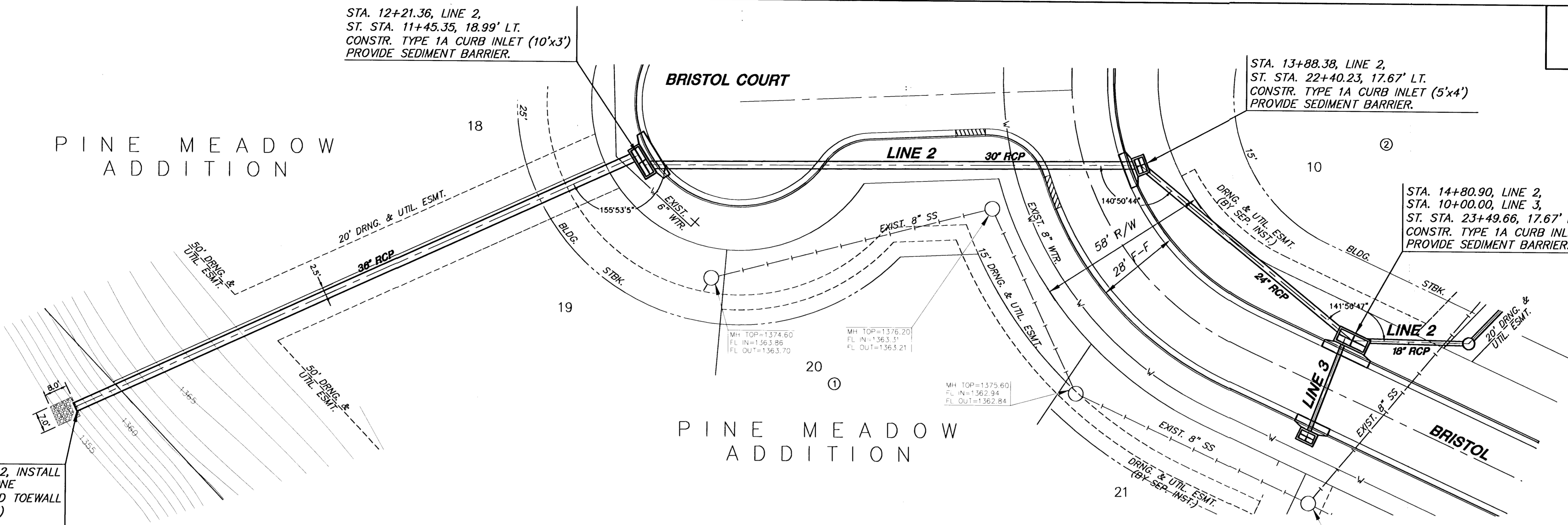
PLAN LINE 2 SCALE: 1"=20'
