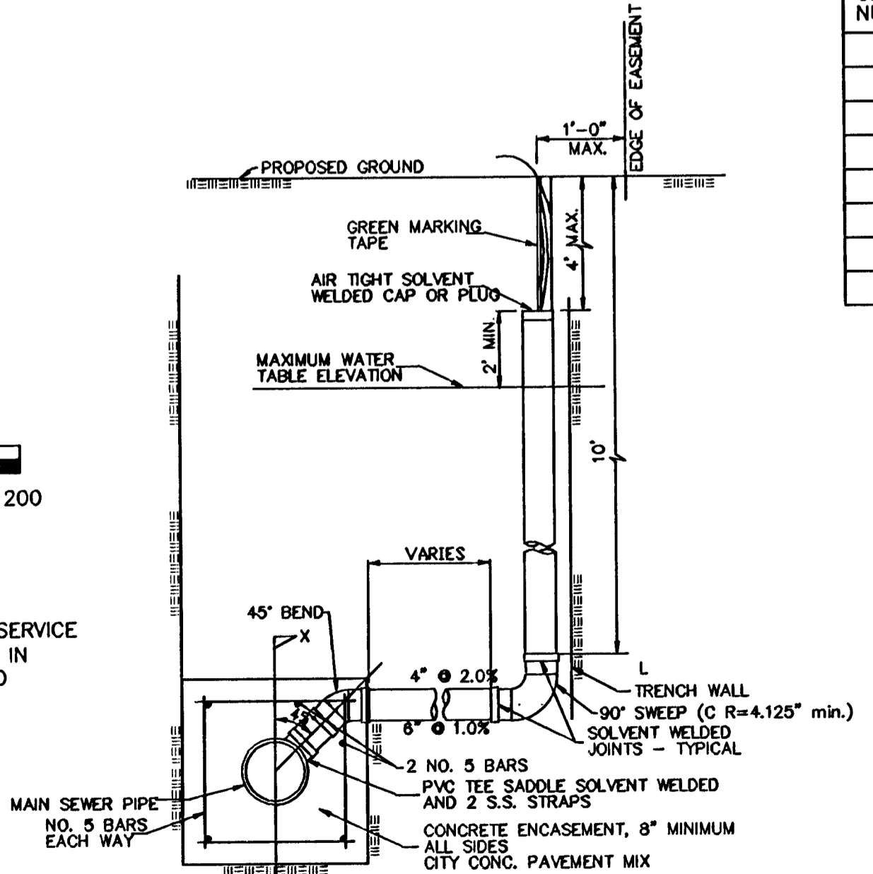
TYPICAL RISER DETAIL
