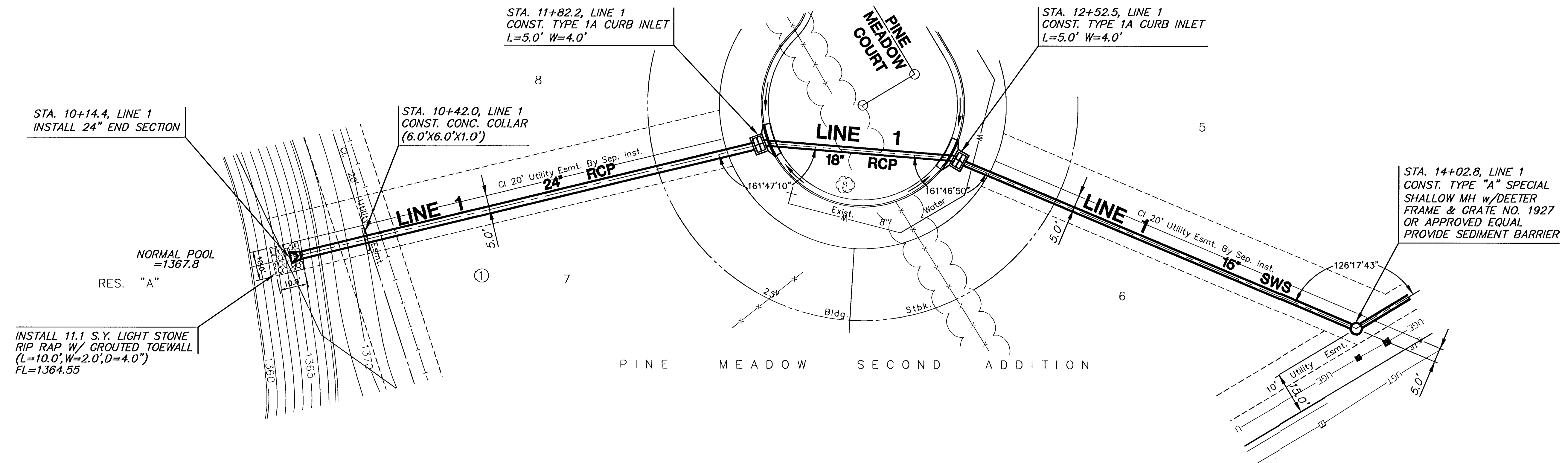
PLAN LINE 1
