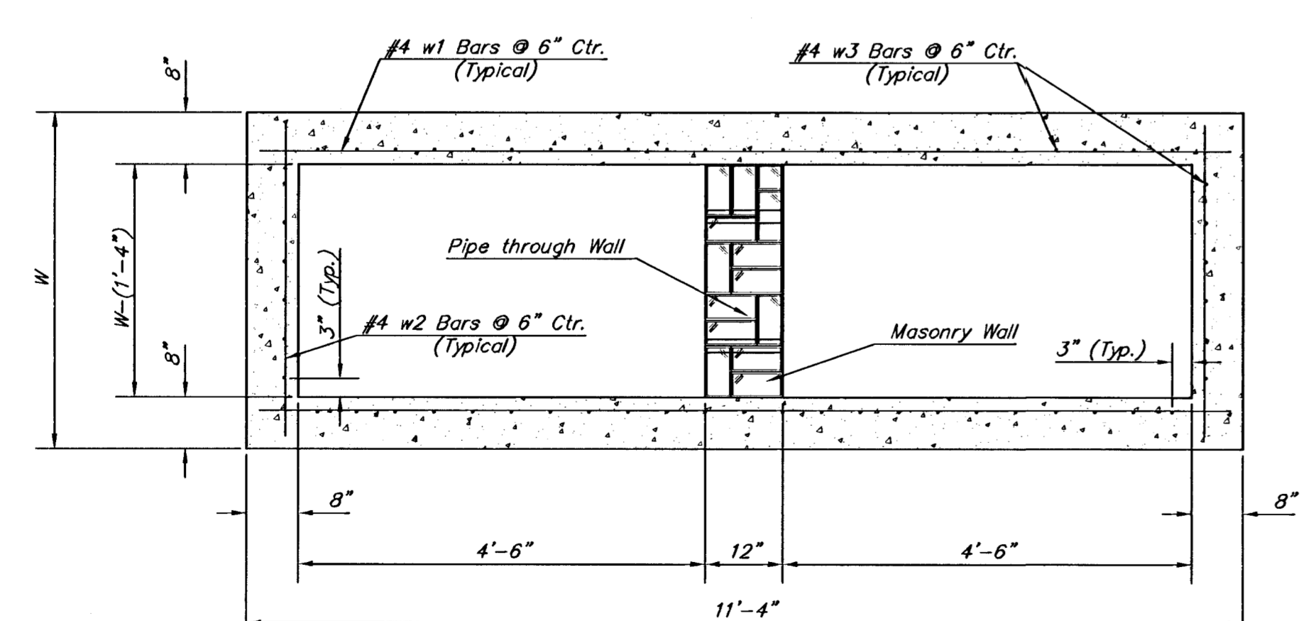
SECTION B-B
