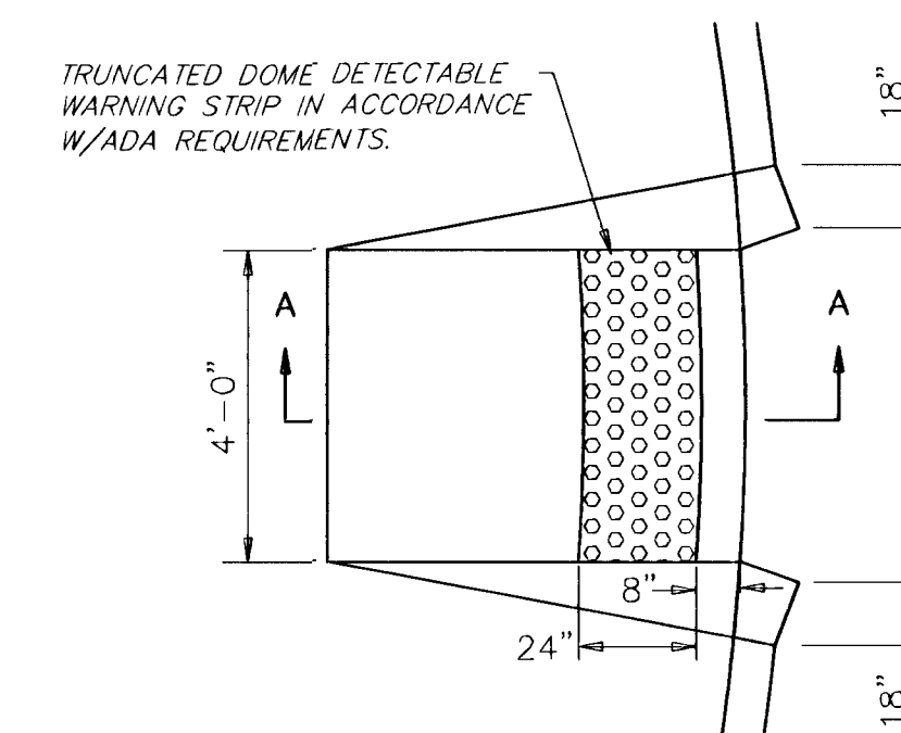
WHEELCHAIR RAMP PLAN VIEW
