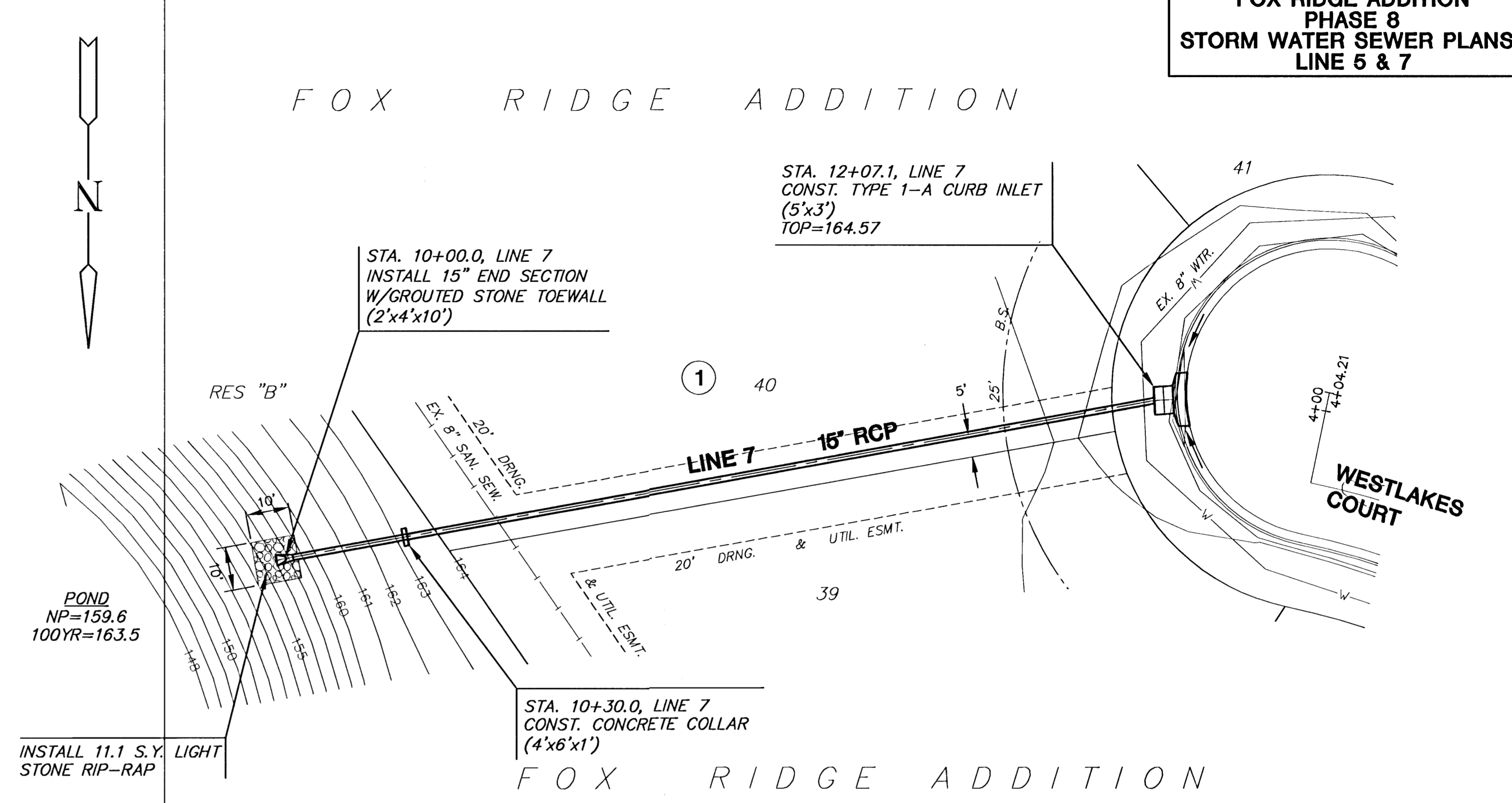
PLAN LINE 7
