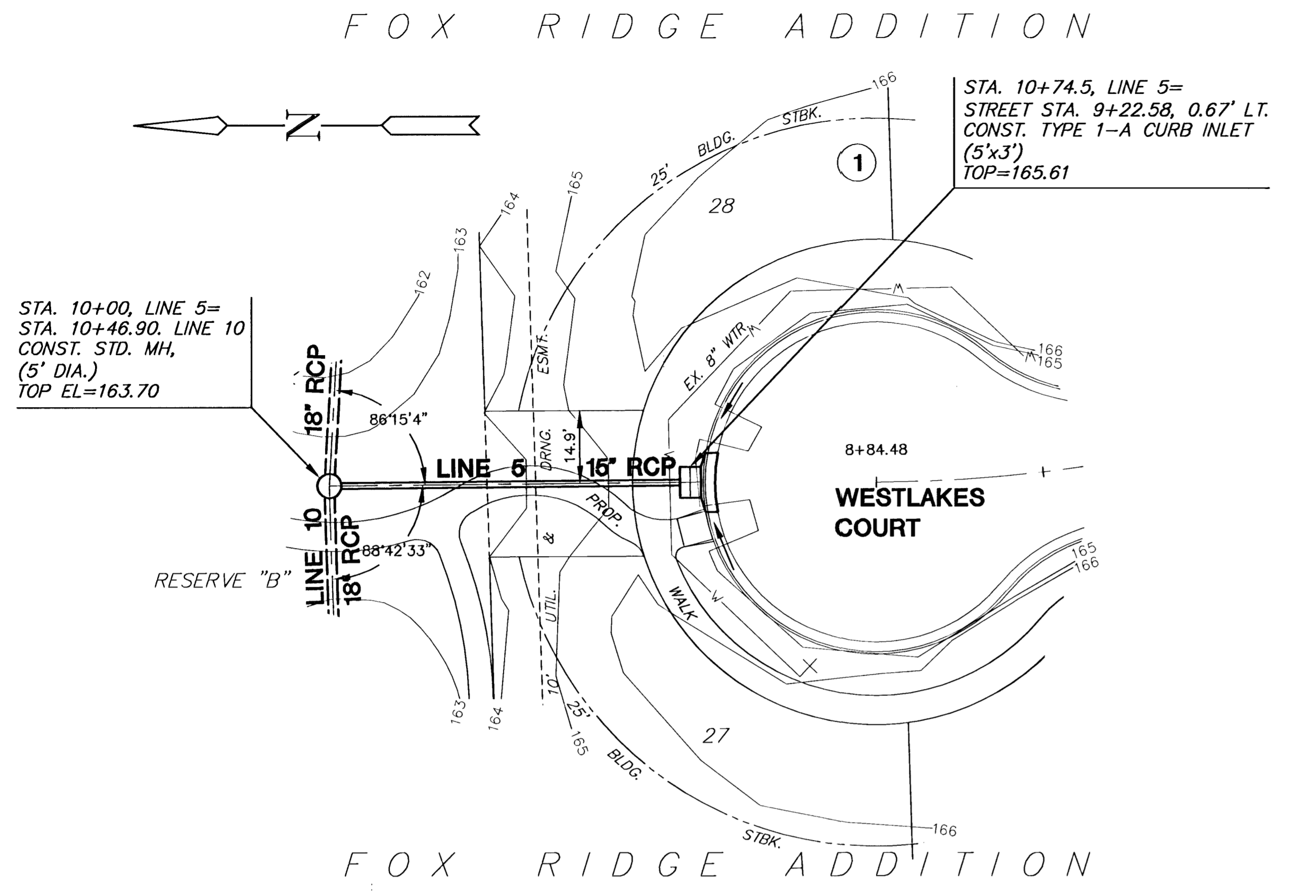
PLAN LINE 5
