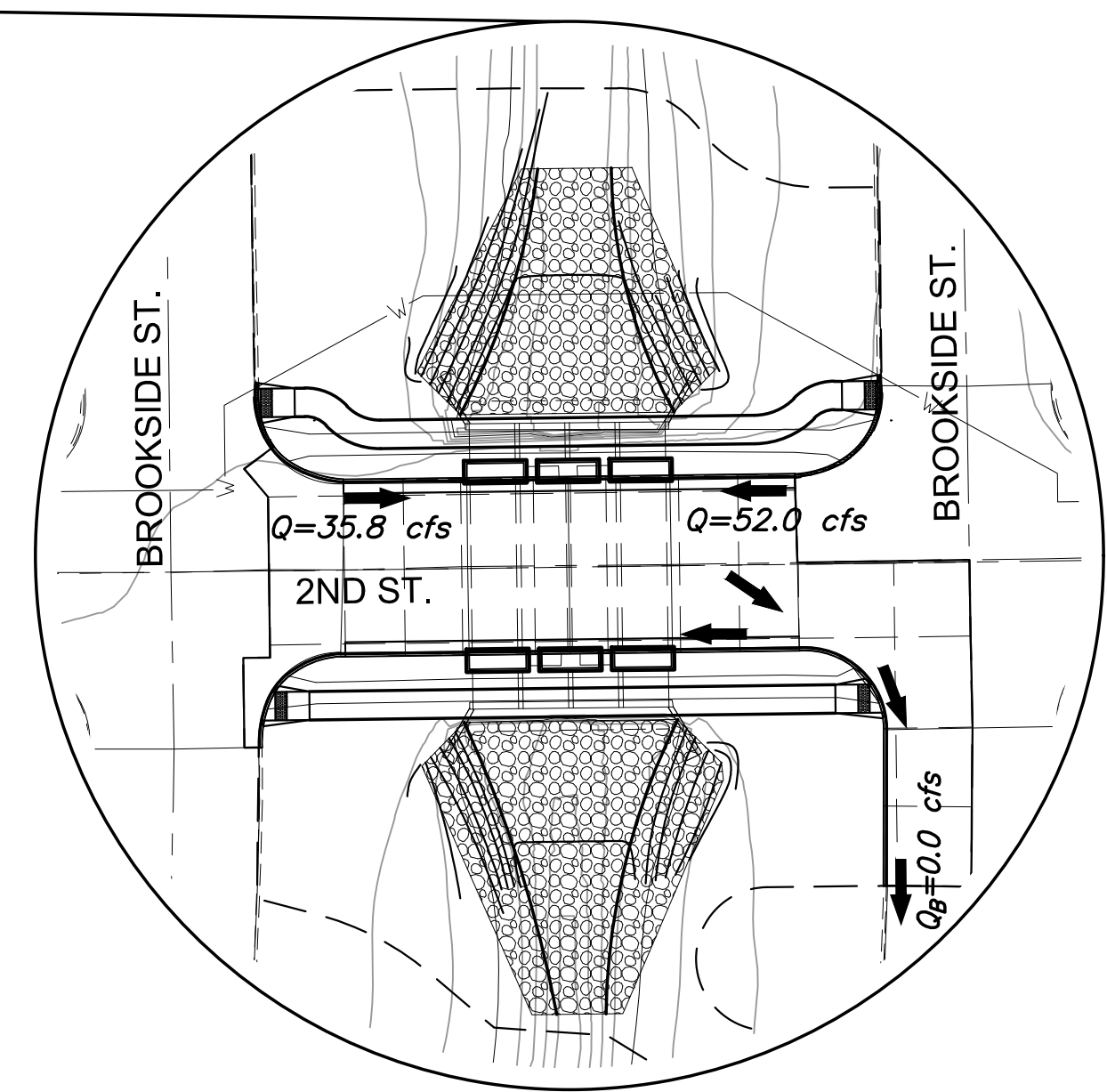
BRIDGE AT 2ND STREET DETAIL
