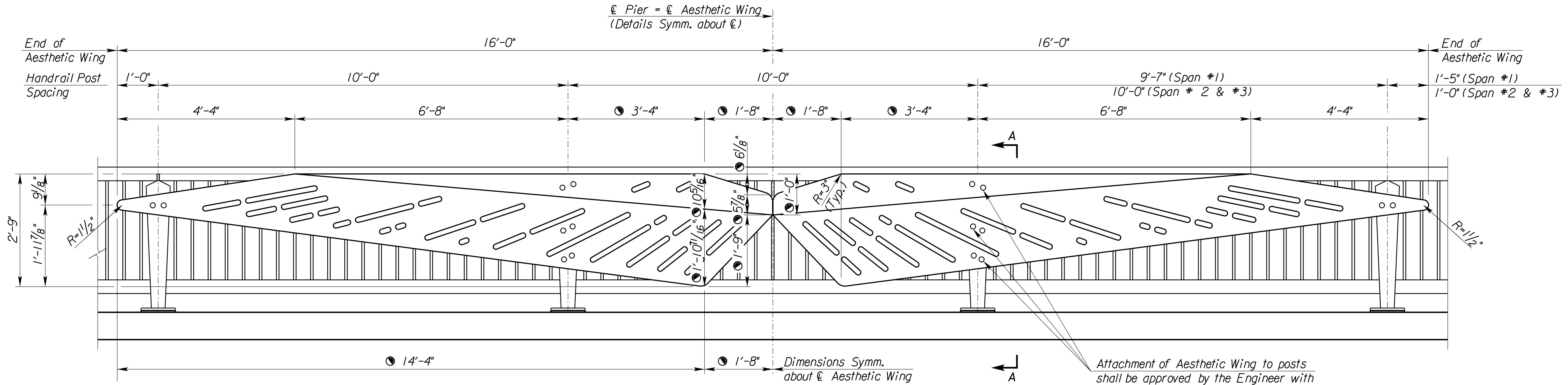
ELEVATION OF AESTHETIC WING (View A-A) (3'-6" Walkway Handrail) (See Sh. #76 for Section A-A.)
