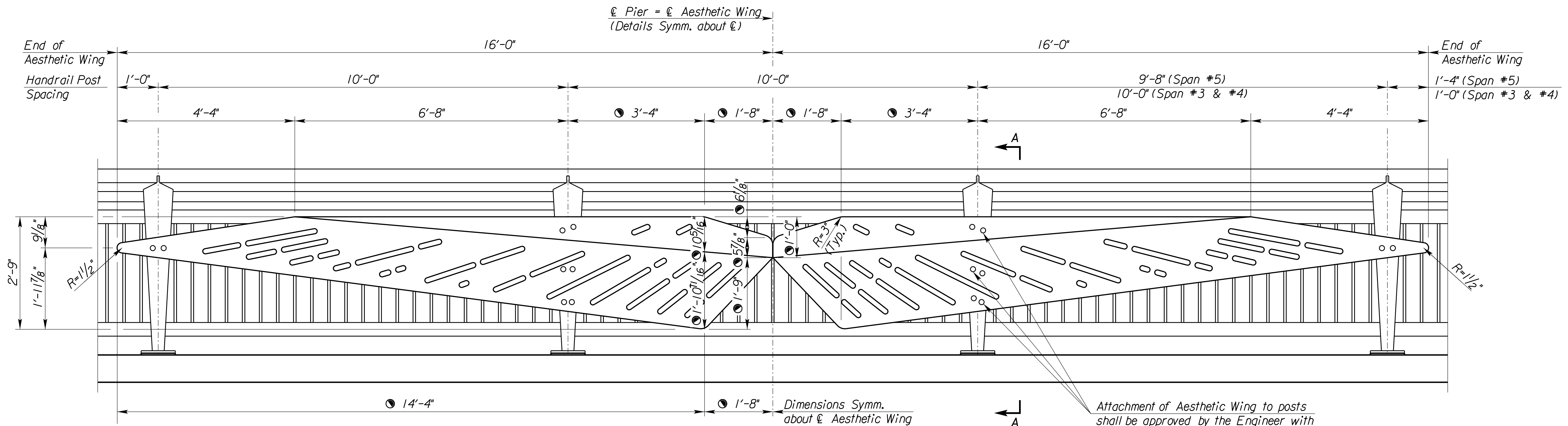
ELEVATION OF AESTHETIC WING (View B-B) (4'-6" Multi-Use Handrail) (See Sh. #77 for Section A-A.)
