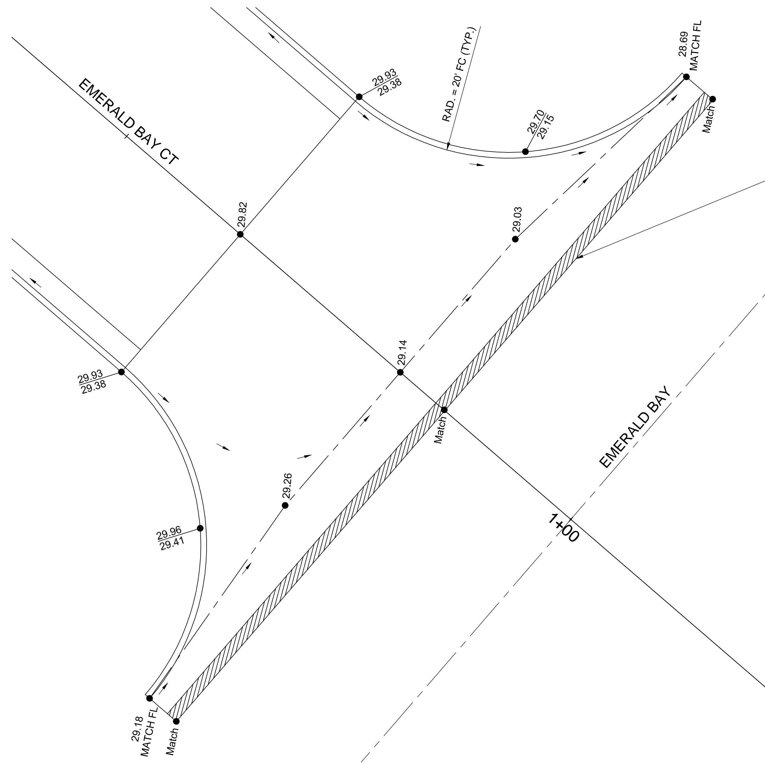
VALLEY GUTTER DETAIL
