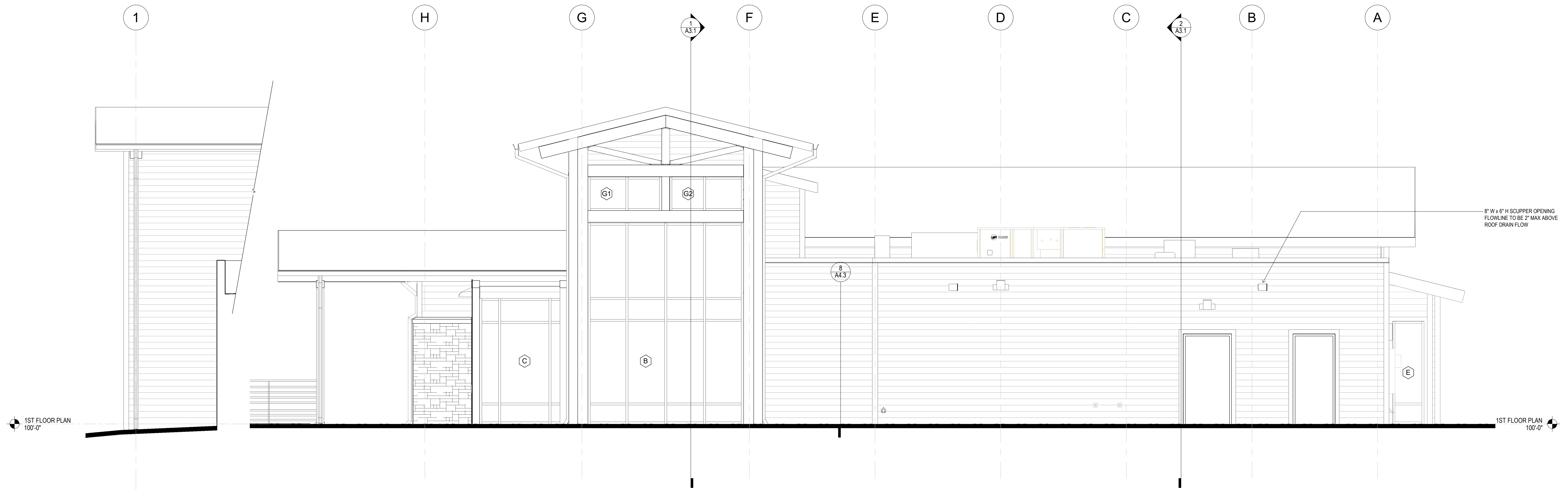
3 HIDDEN ELEVATION 1 1/4" = 1'-0"
