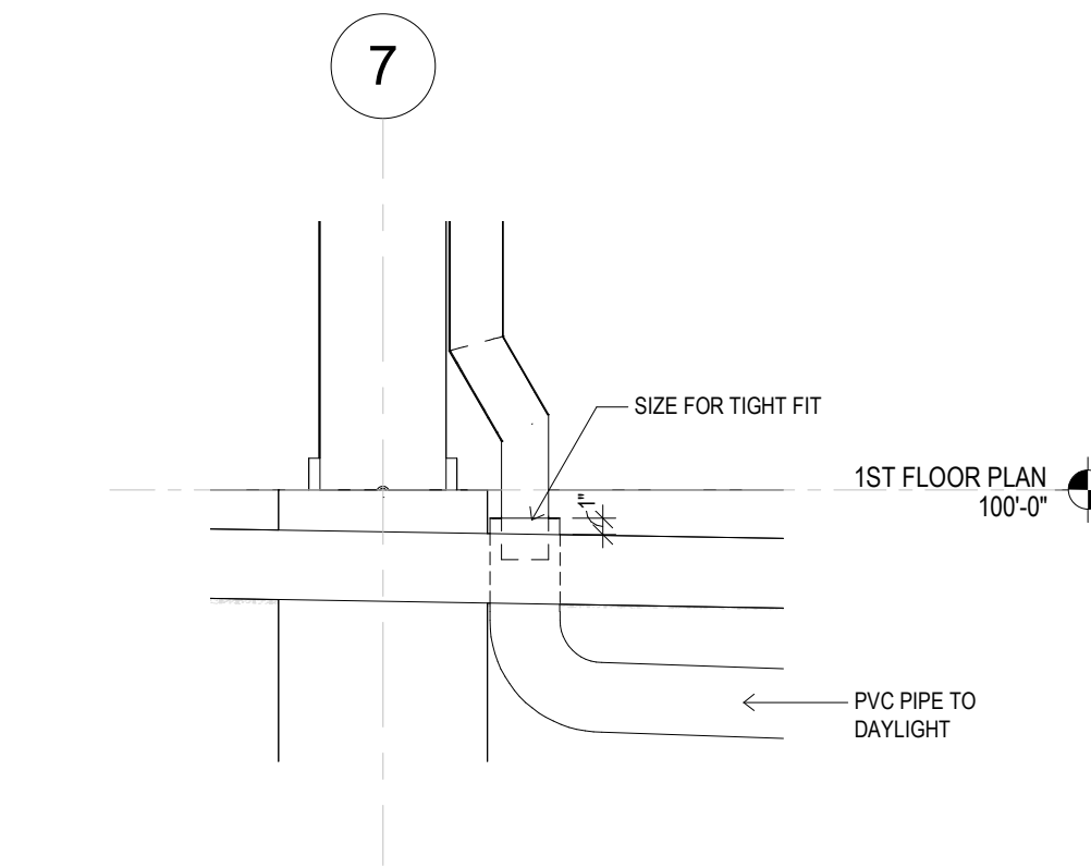
1 PVC PIPE TO DAYLIGHT 1" = 1'-0"
