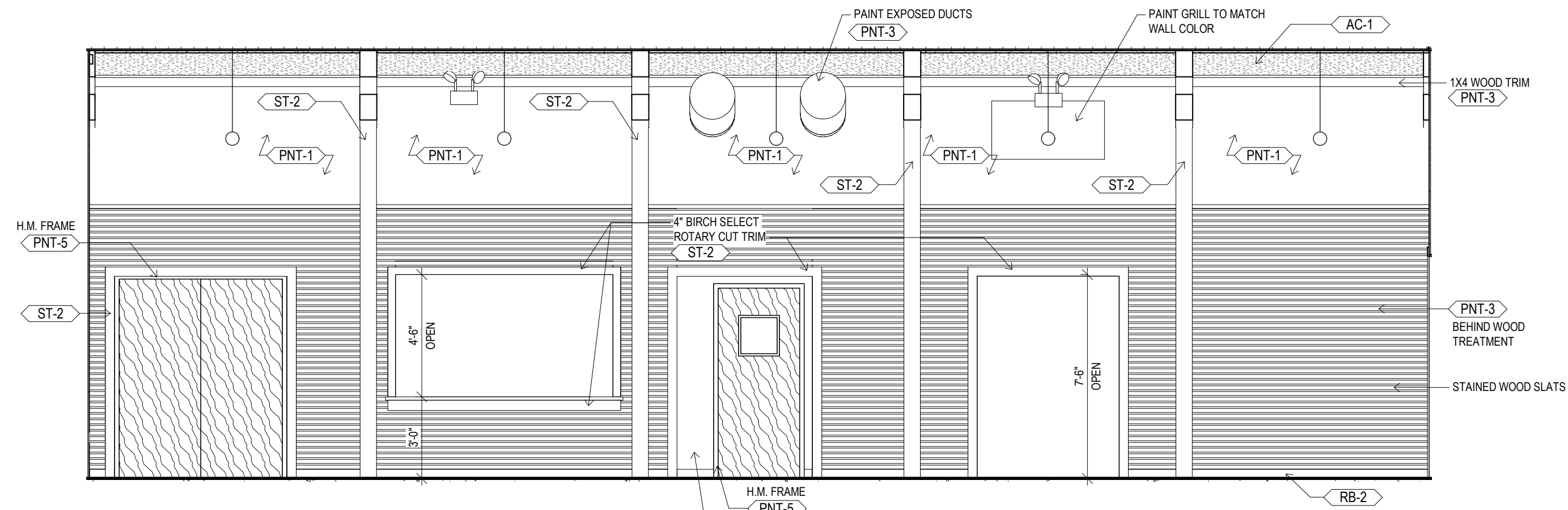
2 GREAT ROOM - NORTH 1/4" = 1'-0"
