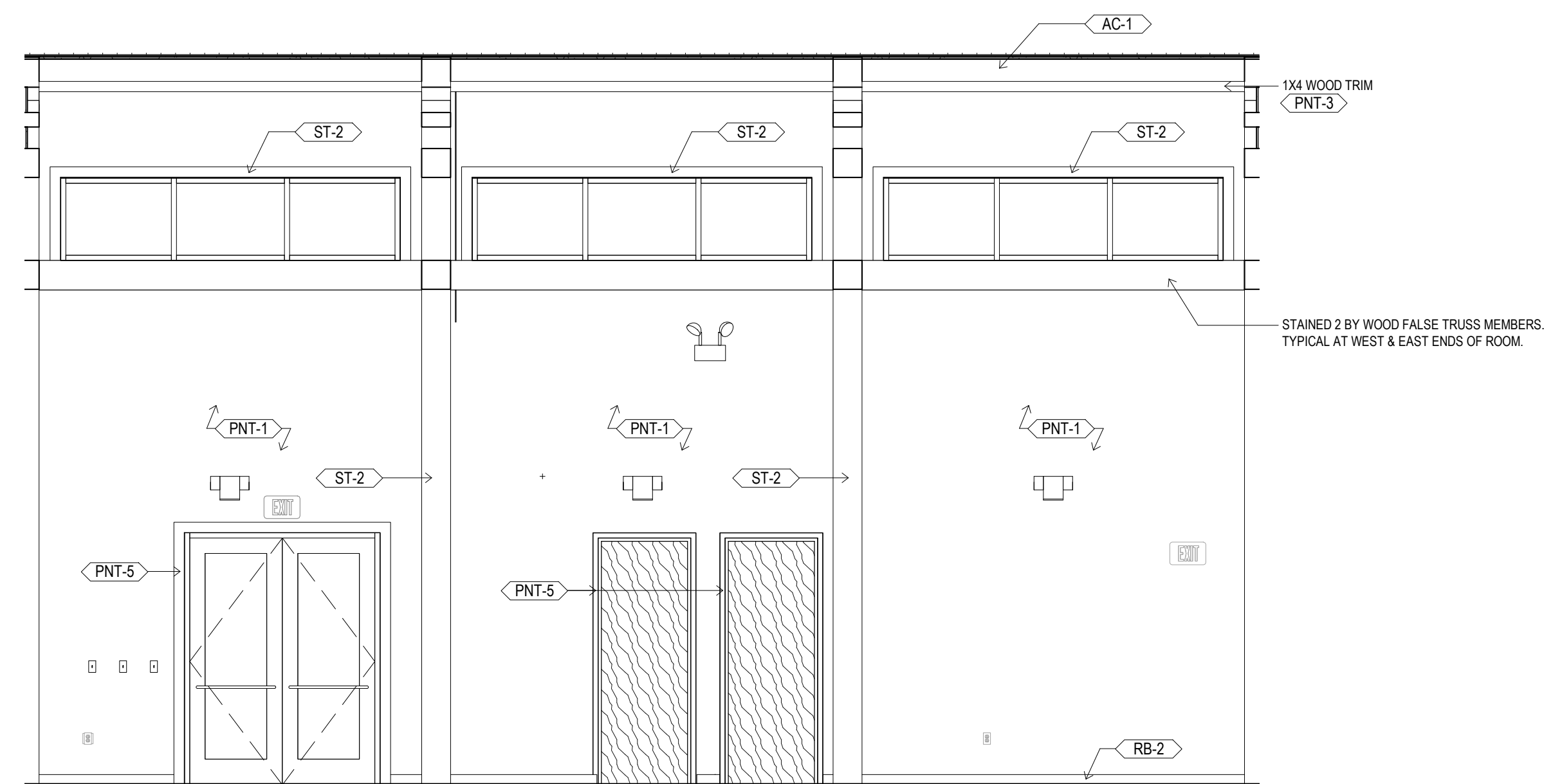
5 GREAT HALL - EAST 1/4" = 1'-0"
