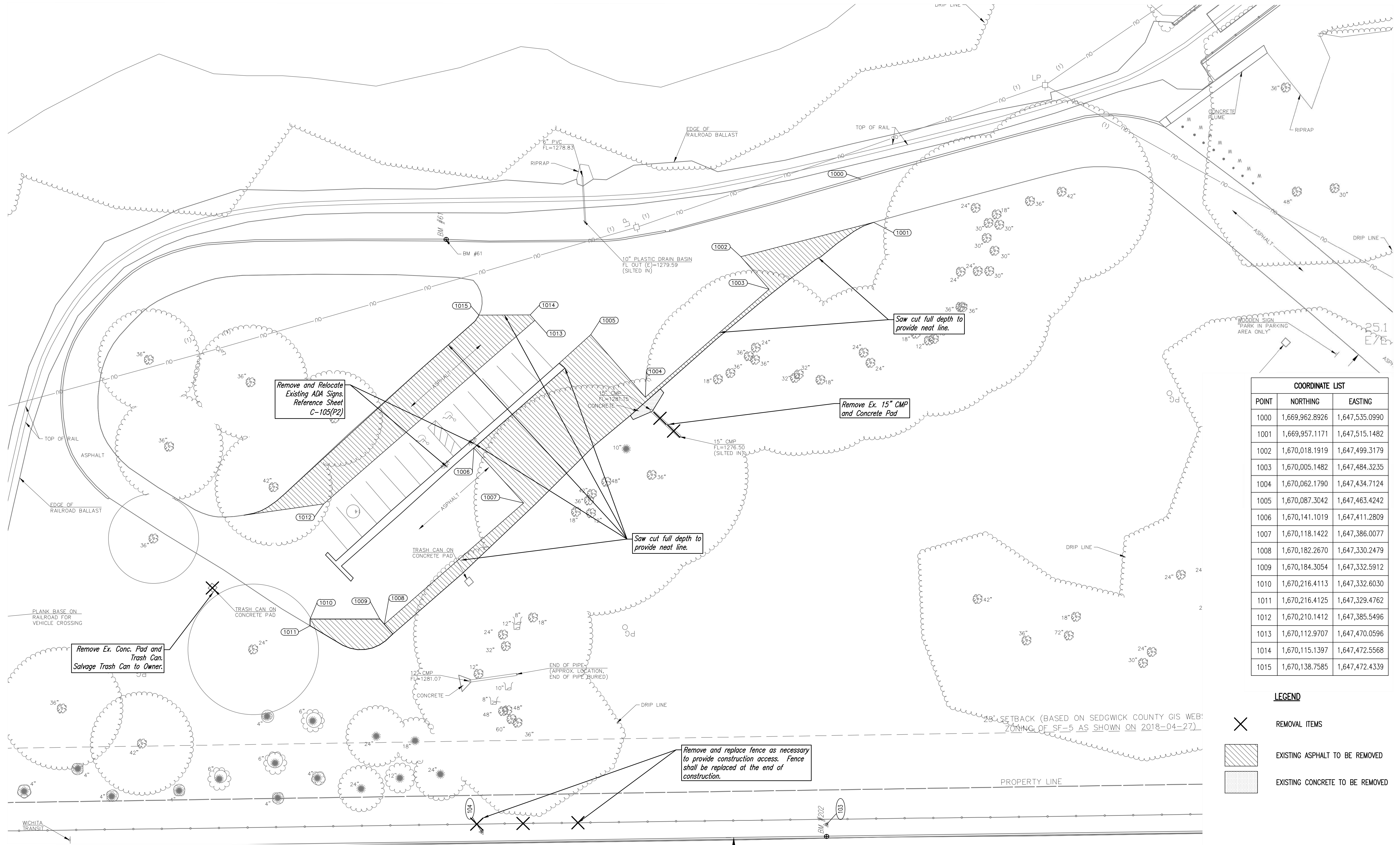
1 PHASE 2 DEMOLITION PLAN 1" = 30' SCALE IN FEET
