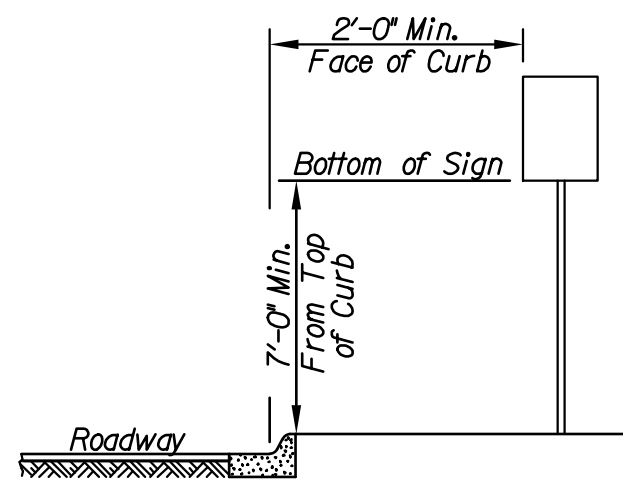
Sign Placement on Roadway Shoulder
