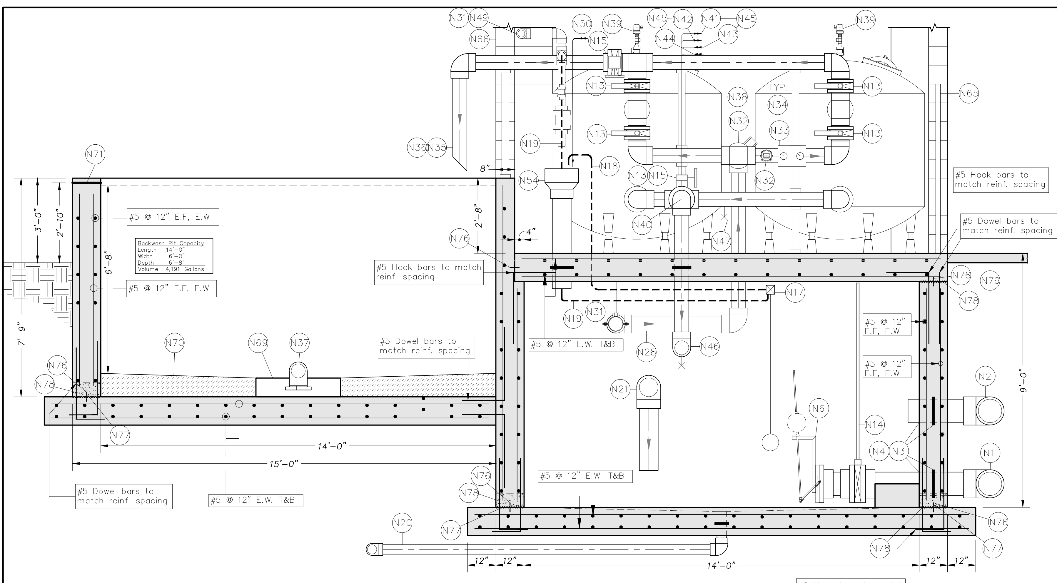
F FILTER AREA IMPROVEMENT PLAN Scale: 1/2"=1'-0"
