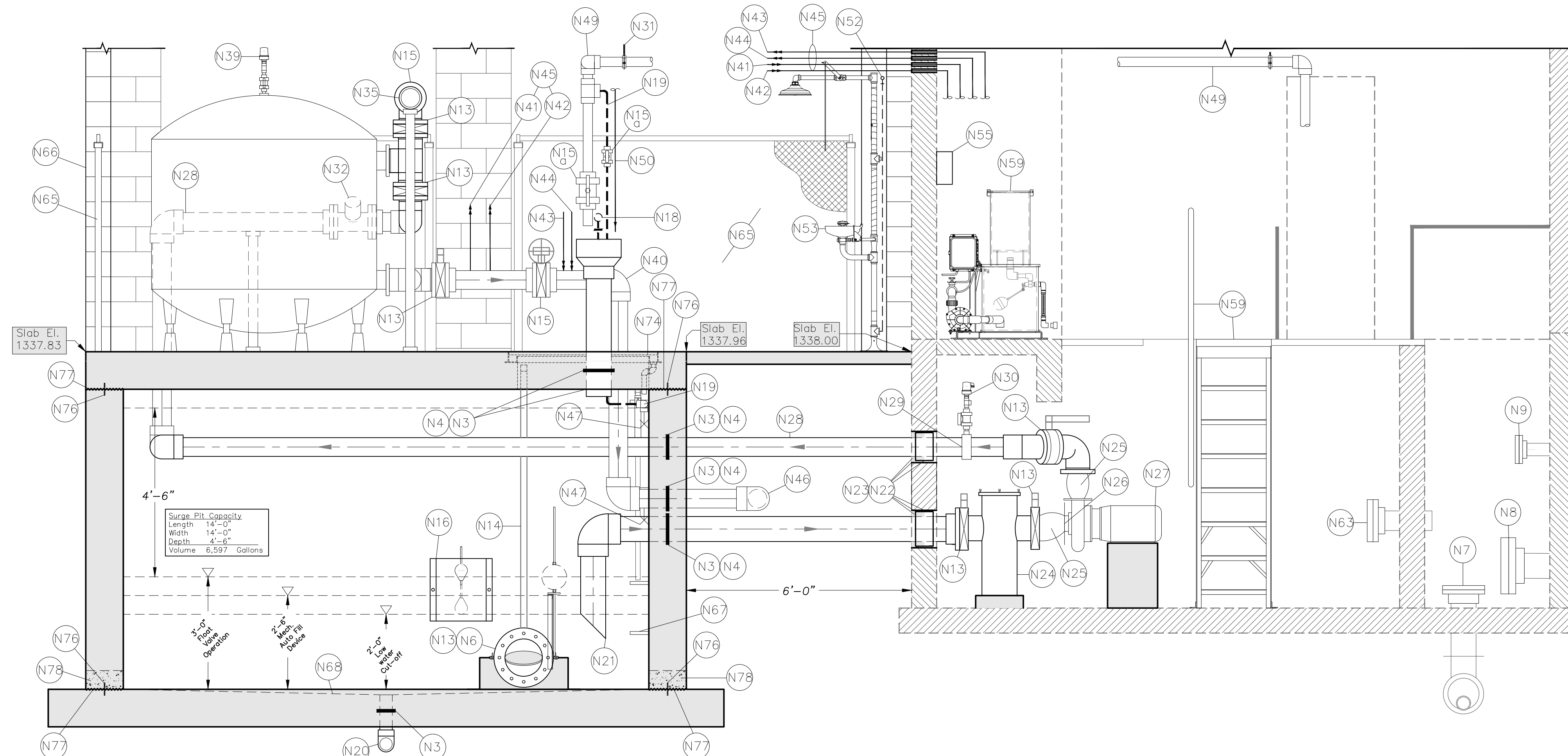
E FILTER AREA IMPROVEMENT PLAN Scale: 1/2"=1'-0"
