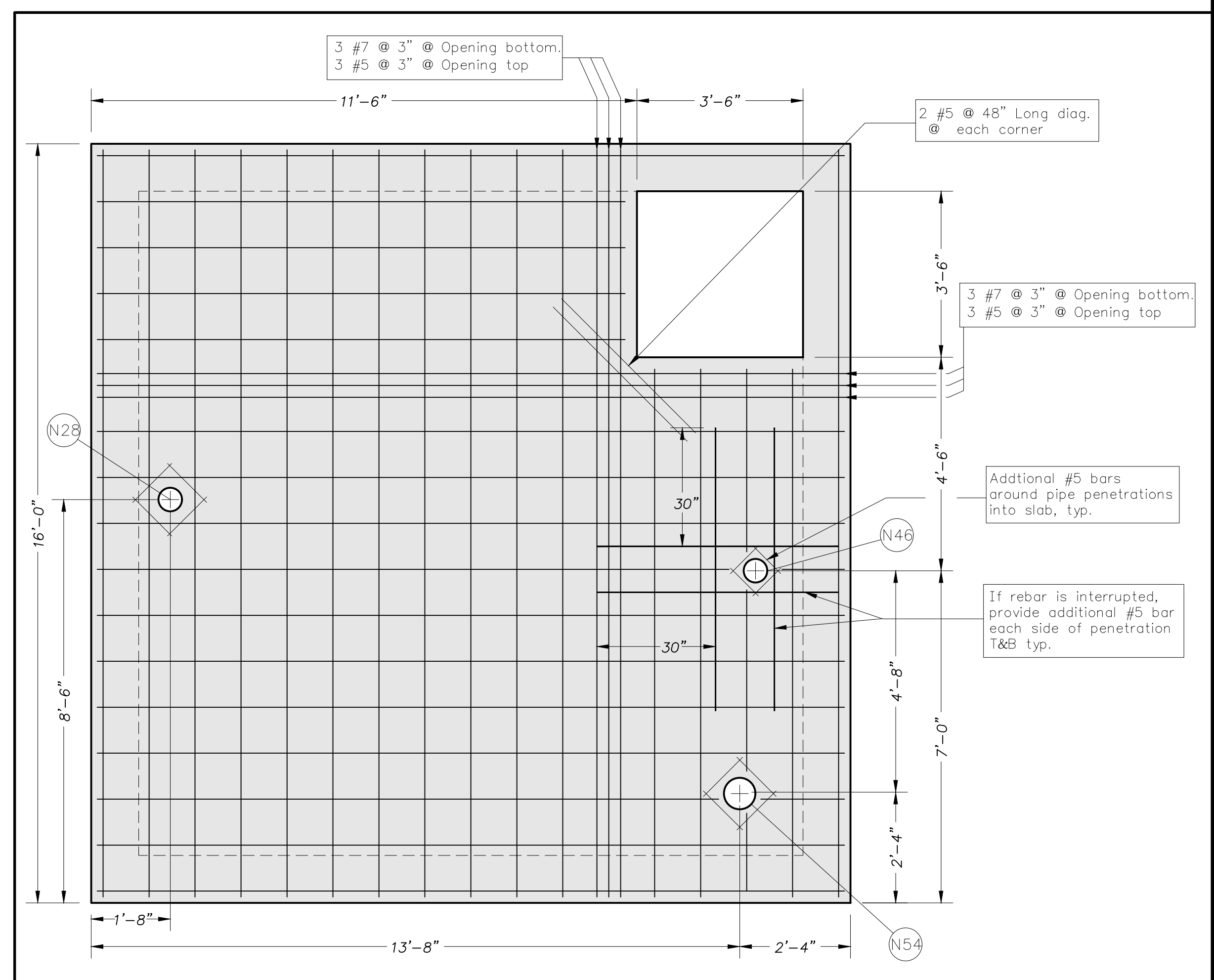
G FILTER AREA IMPROVEMENT PLAN Scale: 1/2"=1'-0"
