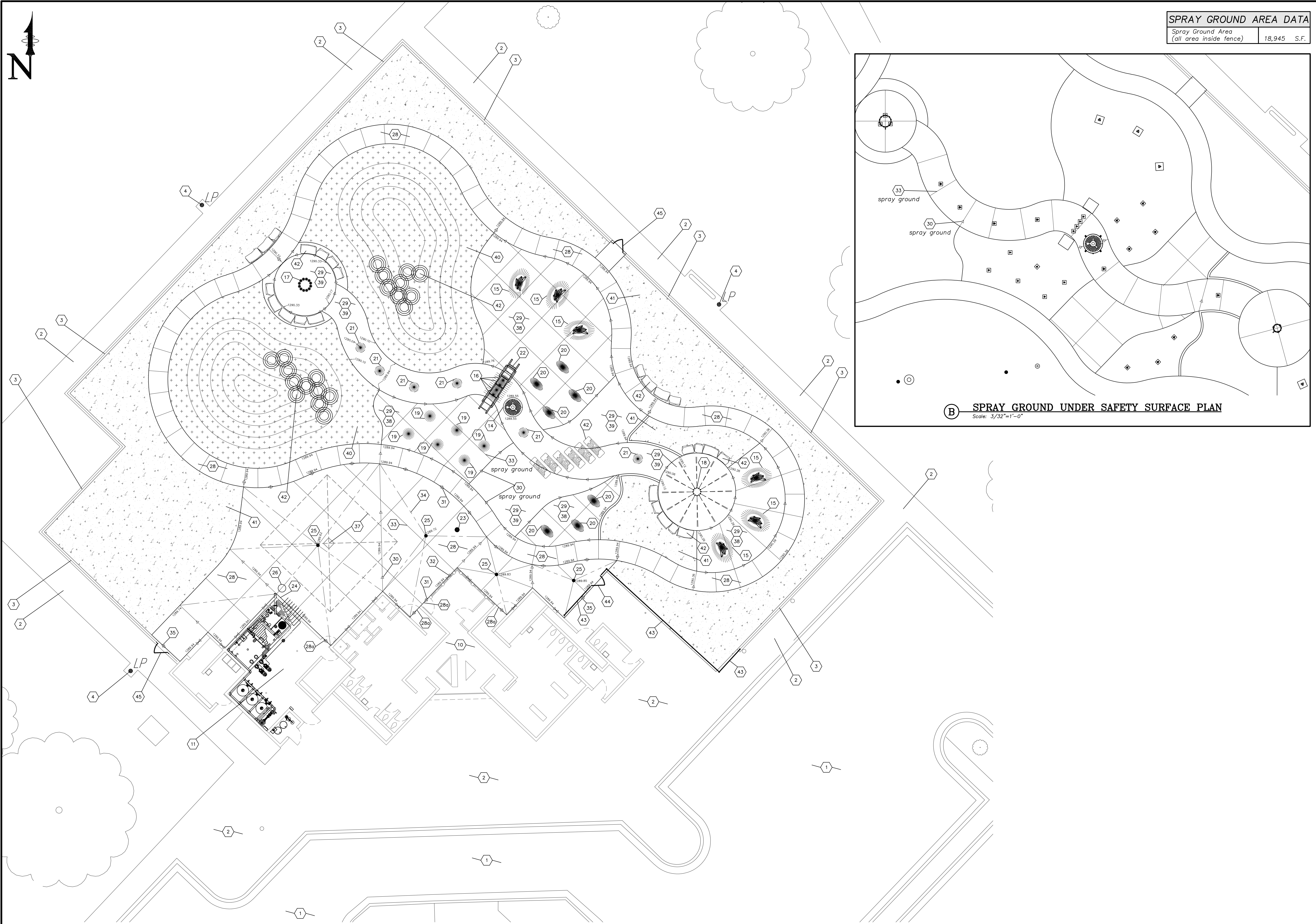
A SPRAY GROUND PLAN Scale: 3/32" = 1'-0"
