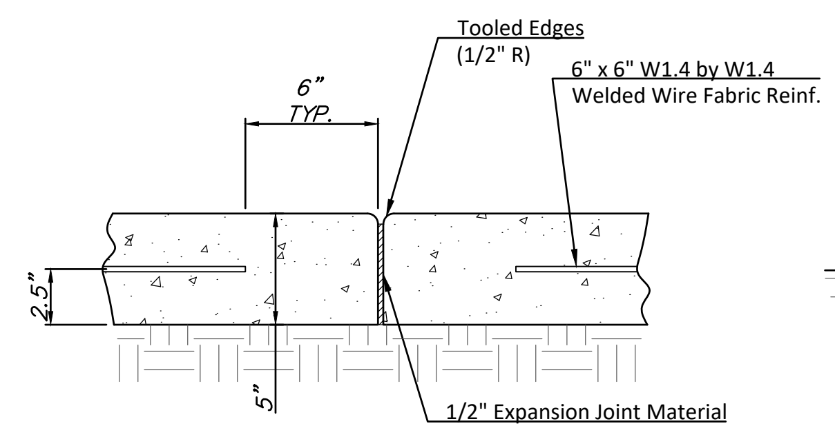
TYPICAL EXPANSION JOINT DETAIL
