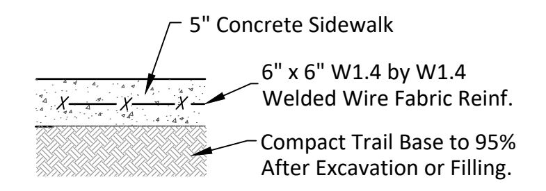
CONCRETE SIDEWALK SECTION
