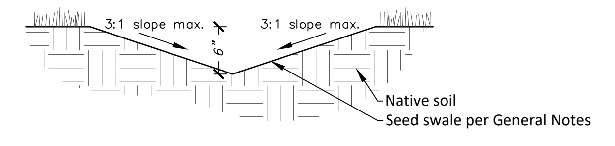
SWALE SECTION
