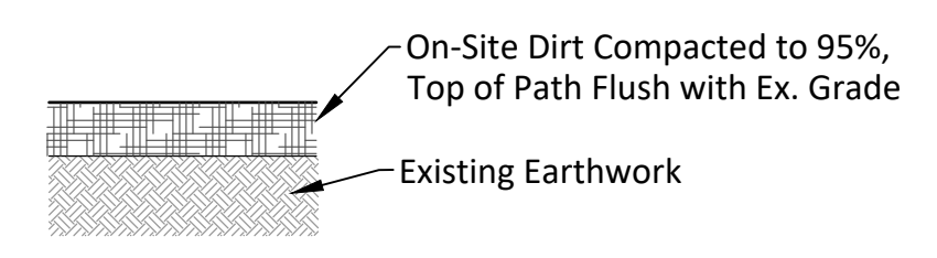
DIRT PATH SECTION
