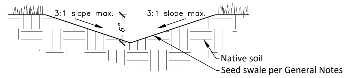
SWALE SECTION
