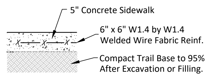
CONCRETE SIDEWALK SECTION
