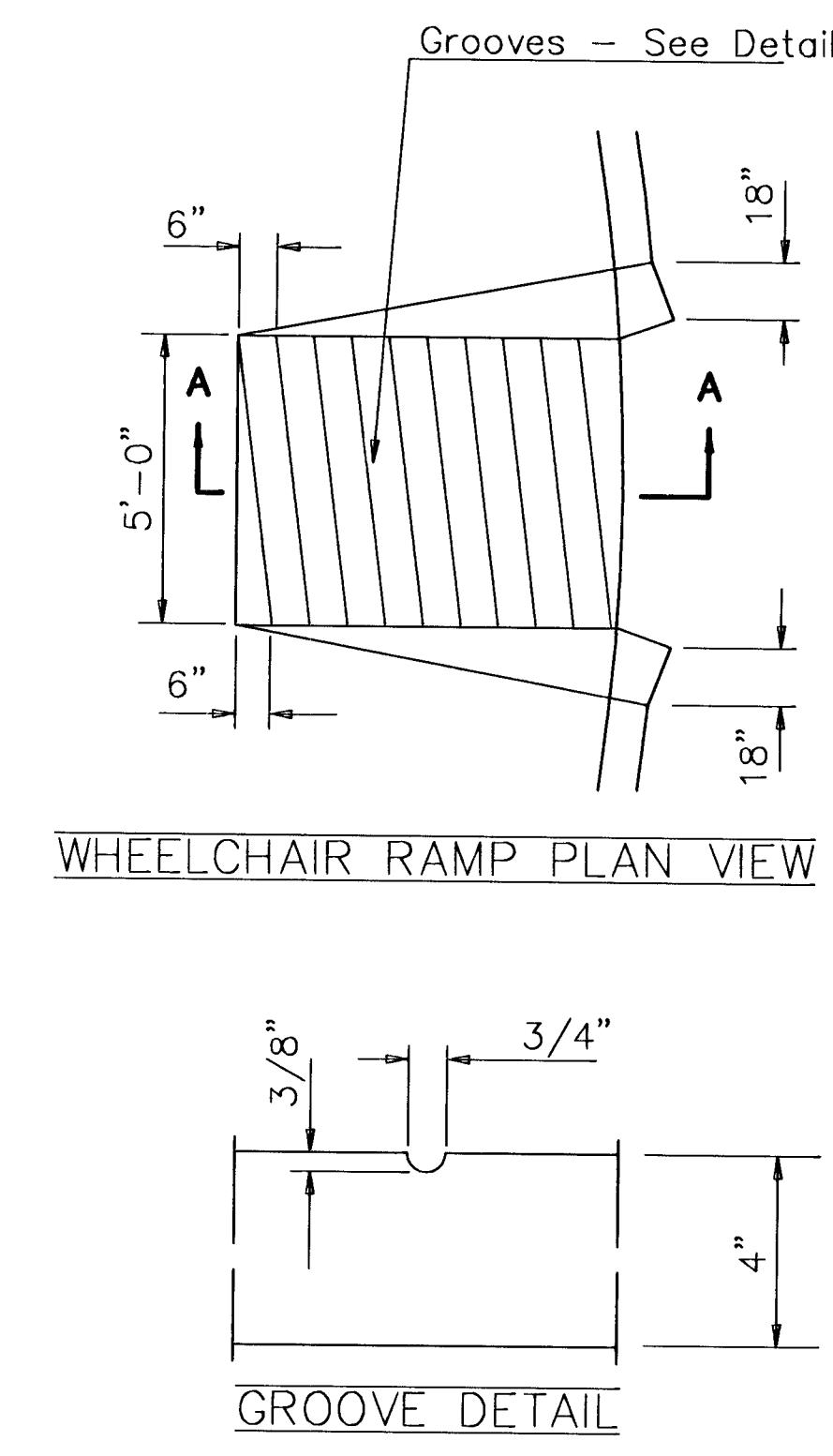
WHEELCHAIR RAMP DETAIL B
