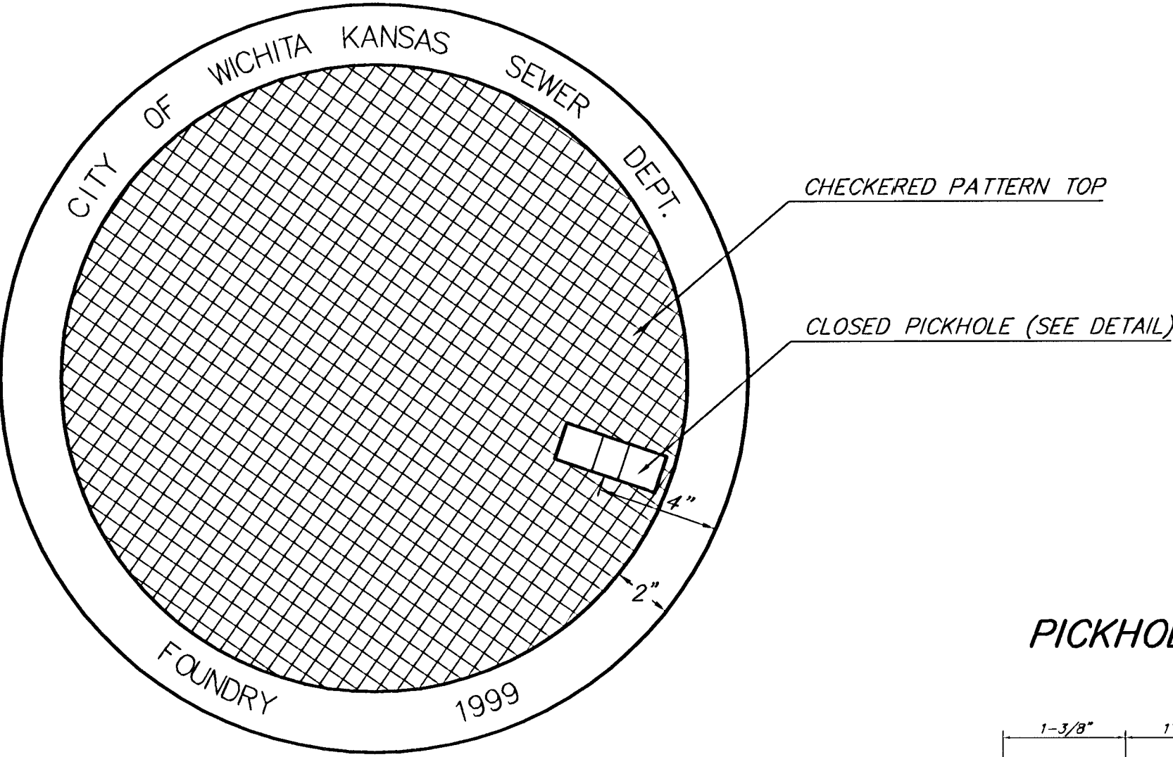
TOP VIEW
