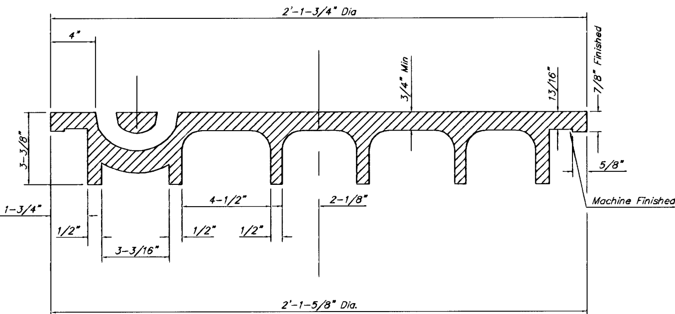
SECTION VIEW
