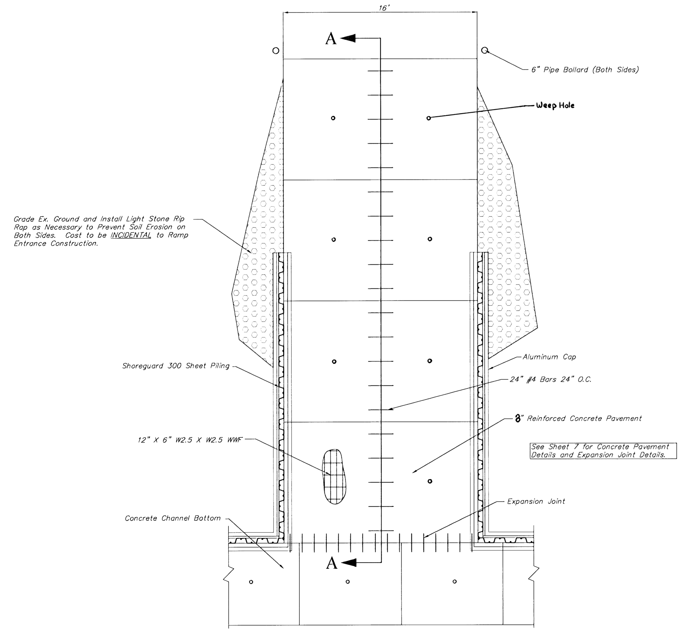
REINF. CONCRETE ENTRANCE RAMP (Not to Scale)
