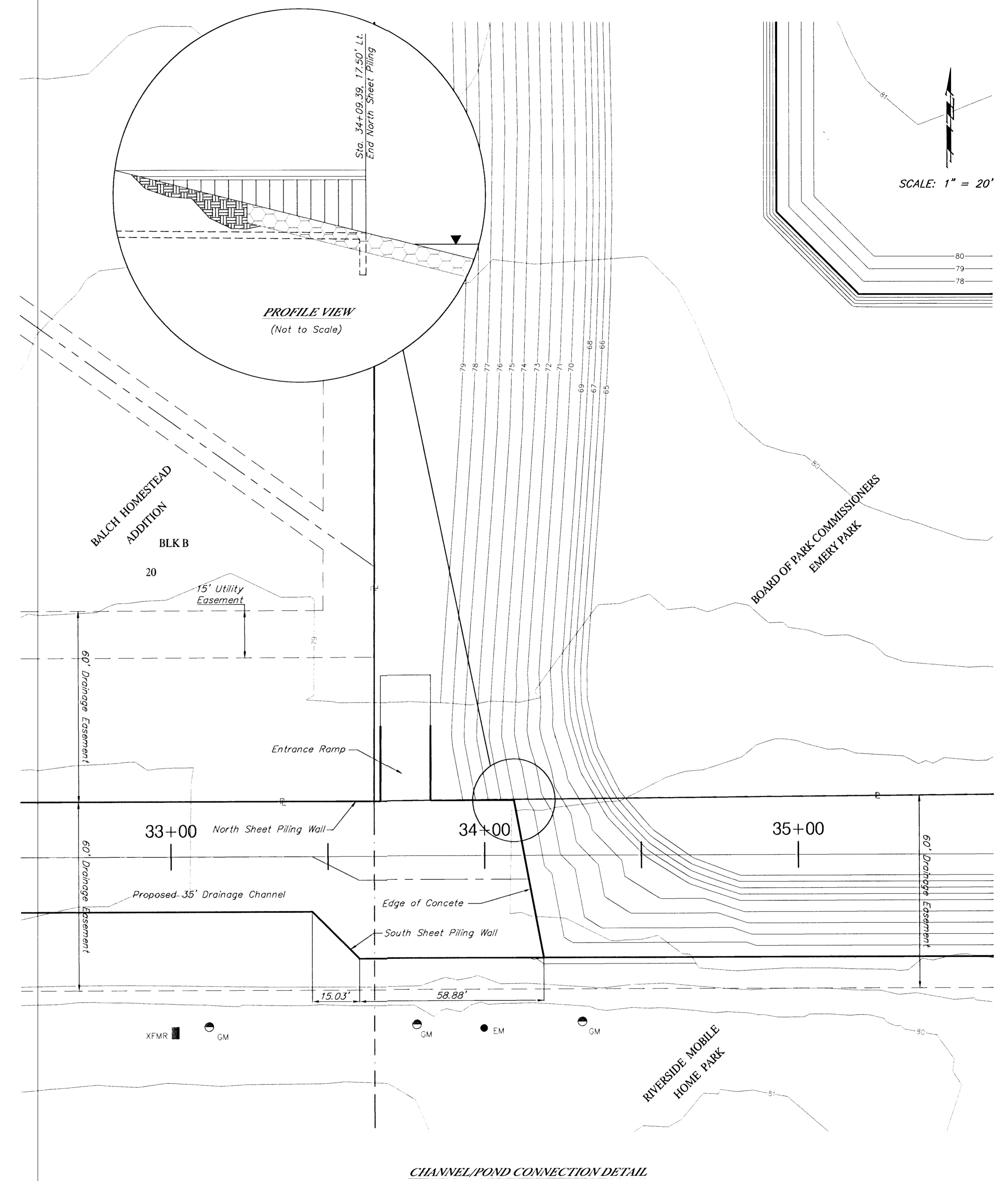
CHANNEL/POND CONNECTION DETAIL
