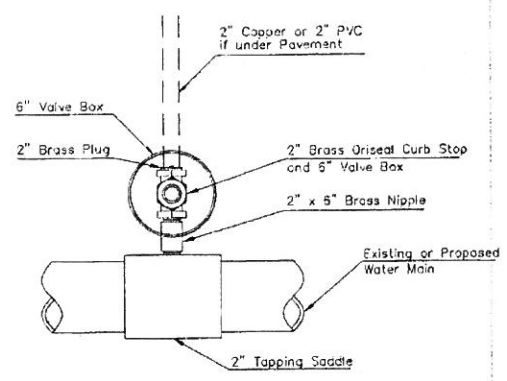
2" SERVICE OUTLET ASSEMBLY TOP VIEW
