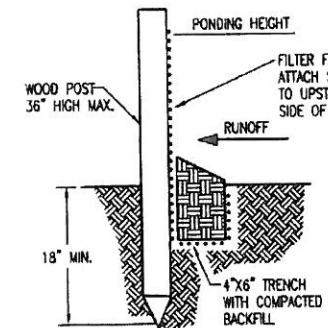
SILT FENCE BARRIERS
