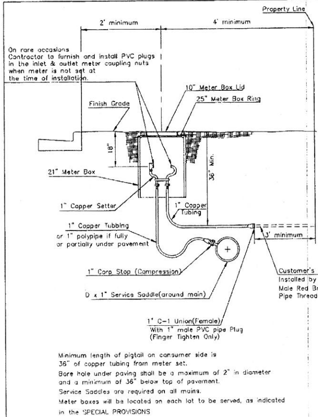
TYPICAL 1" METER SETTING
