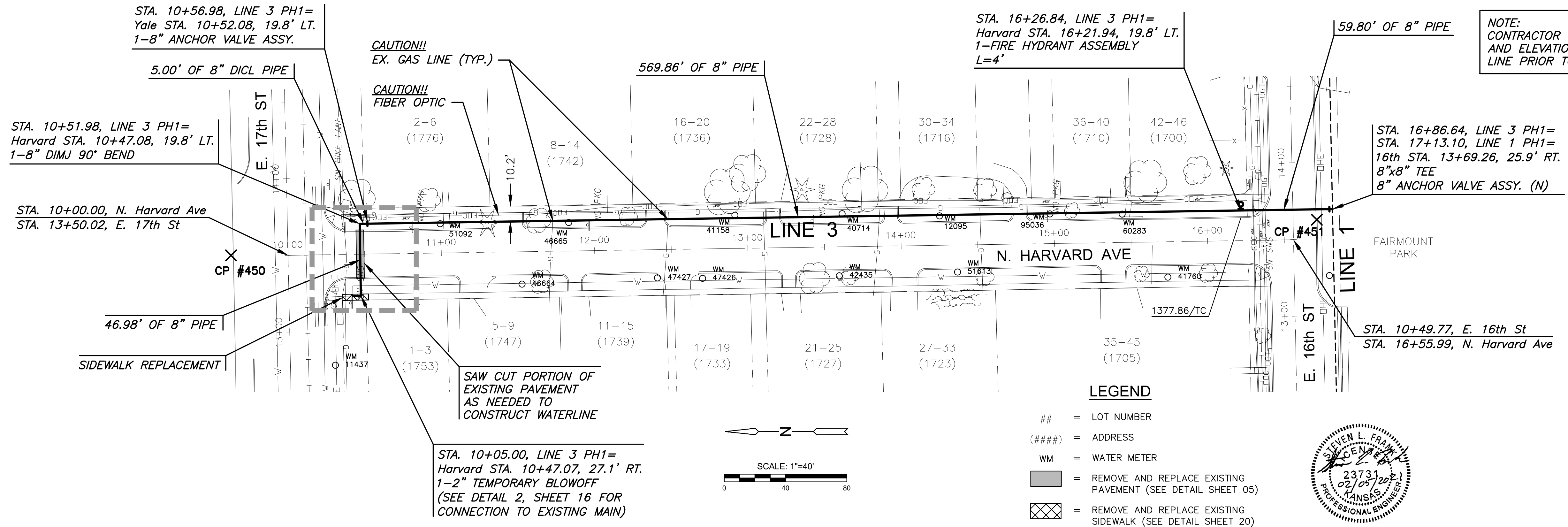
PLAN WTR LINE 3 PROFILE WTR LINE 3
