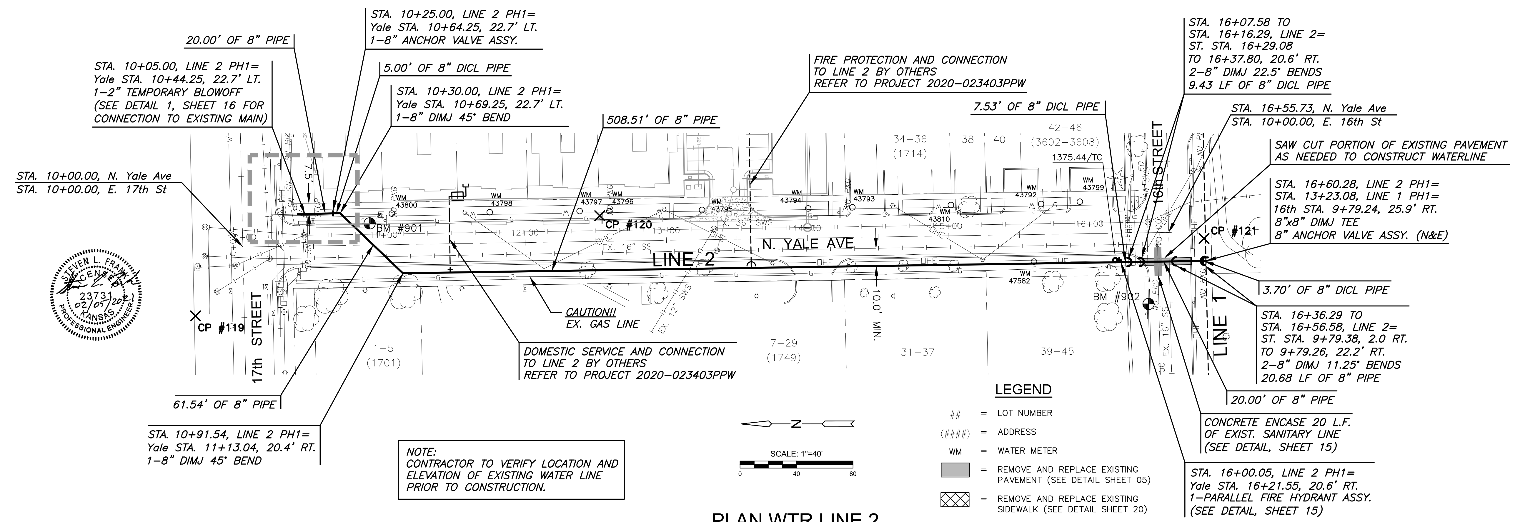
PLAN WTR LINE 2 PROFILE WTR LINE 2
