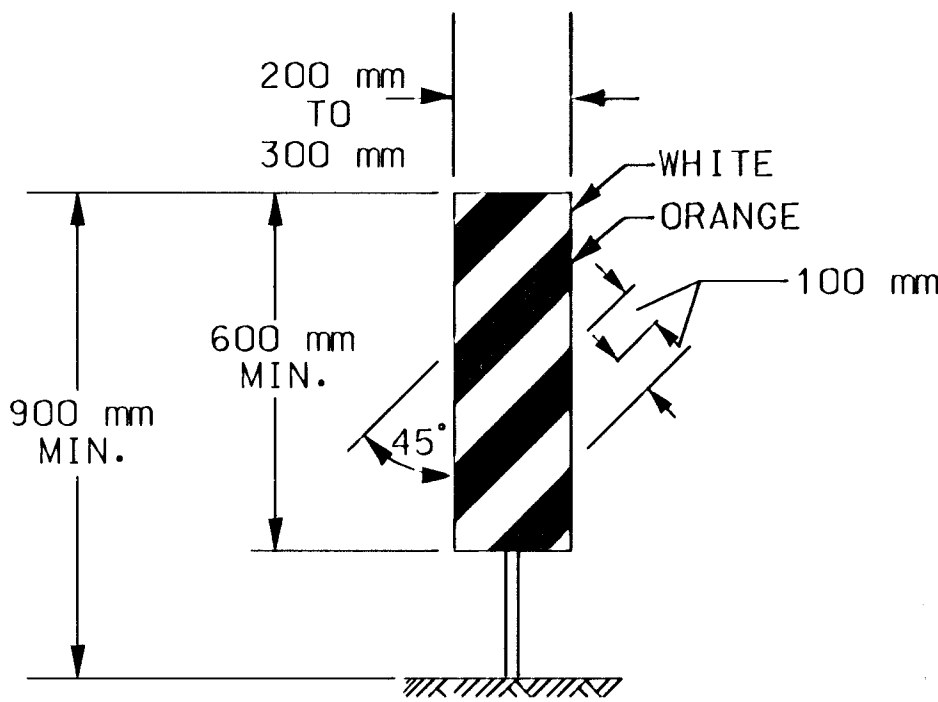
VERTICAL PANEL
