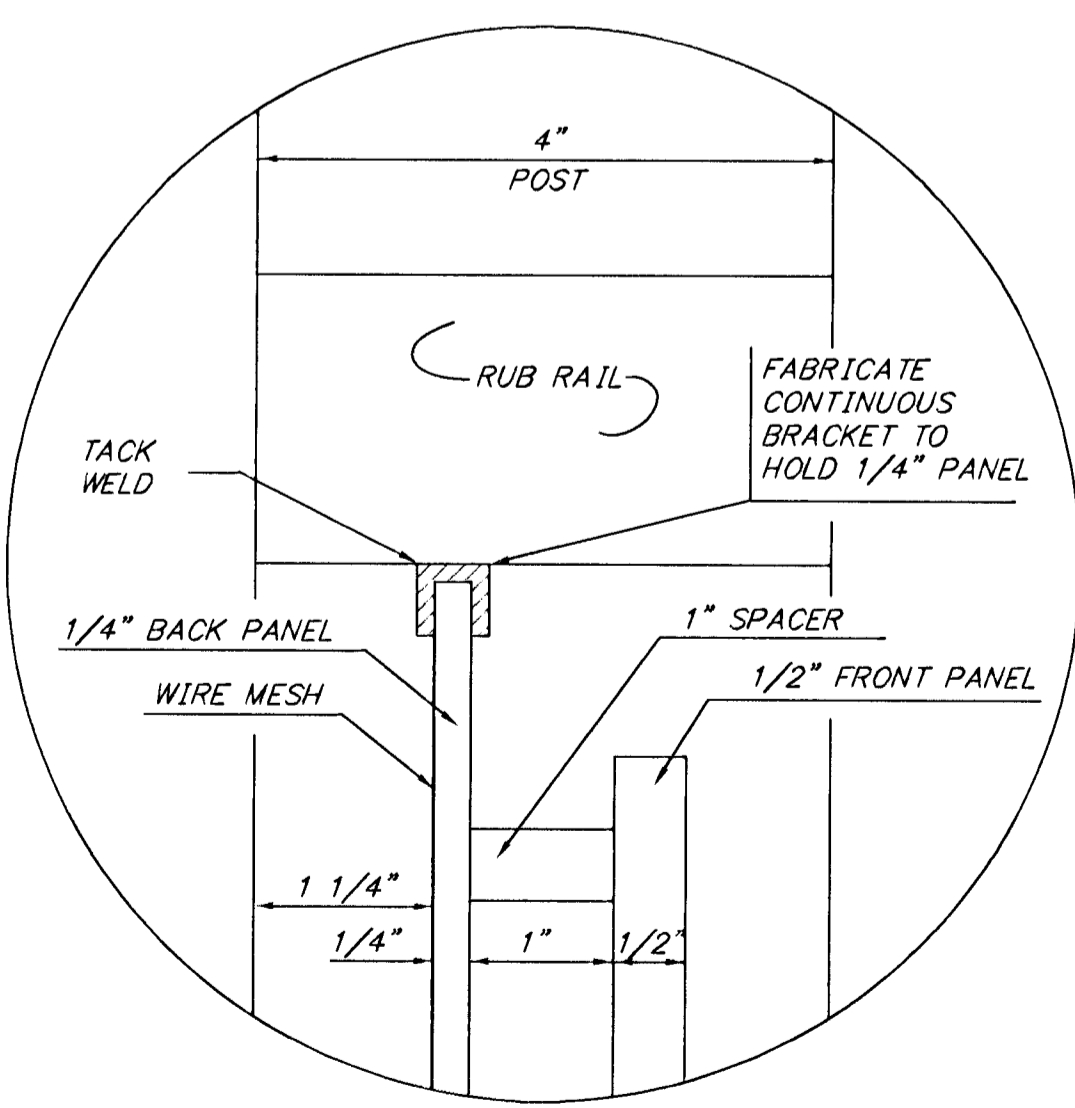
PANEL INSERT DETAIL NO SCALE
