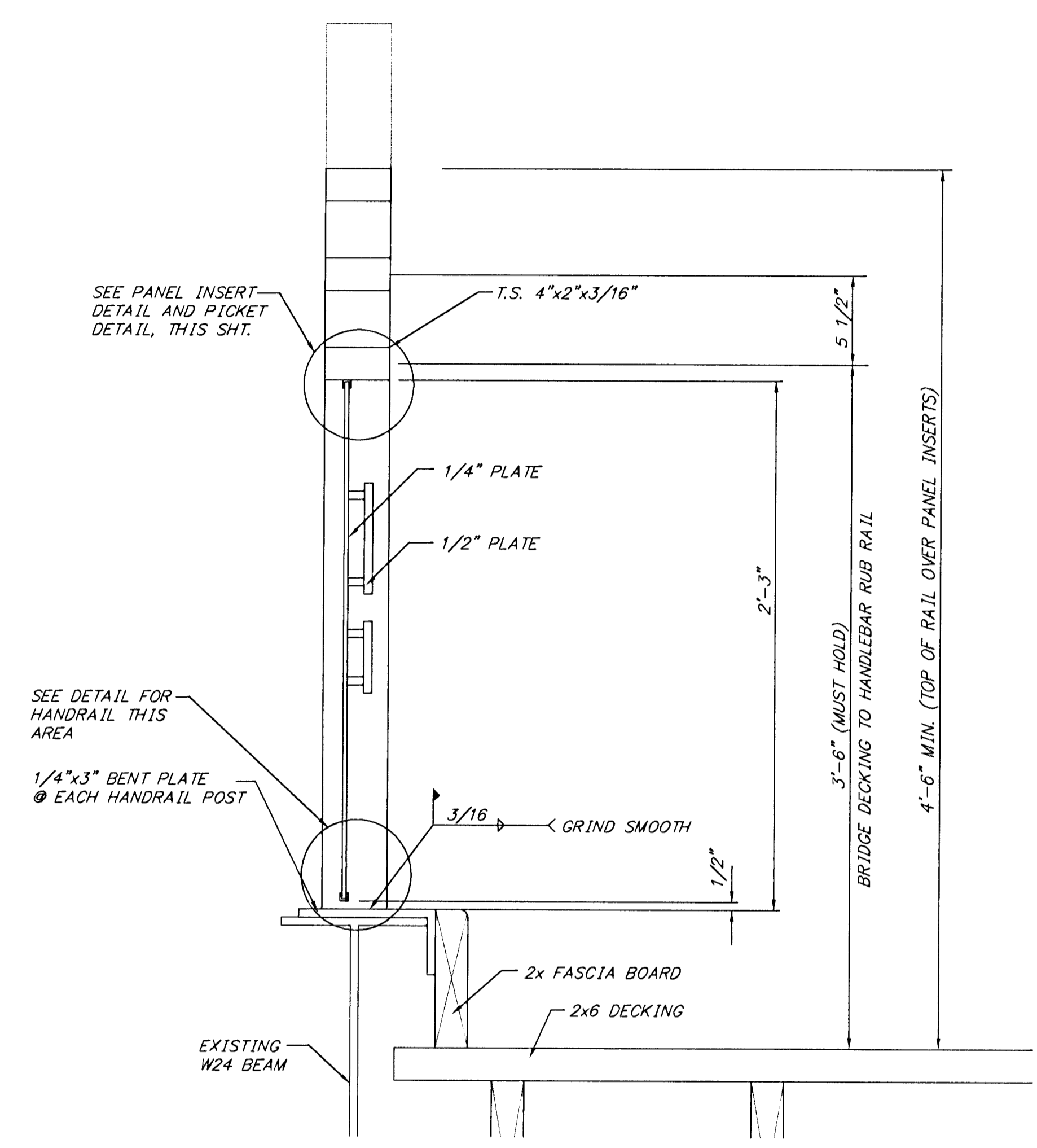
HANDRAIL SECTION NO SCALE
