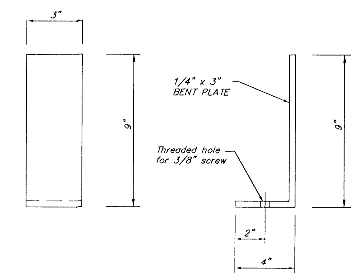
HANDRAIL BASE PLATE NO SCALE
