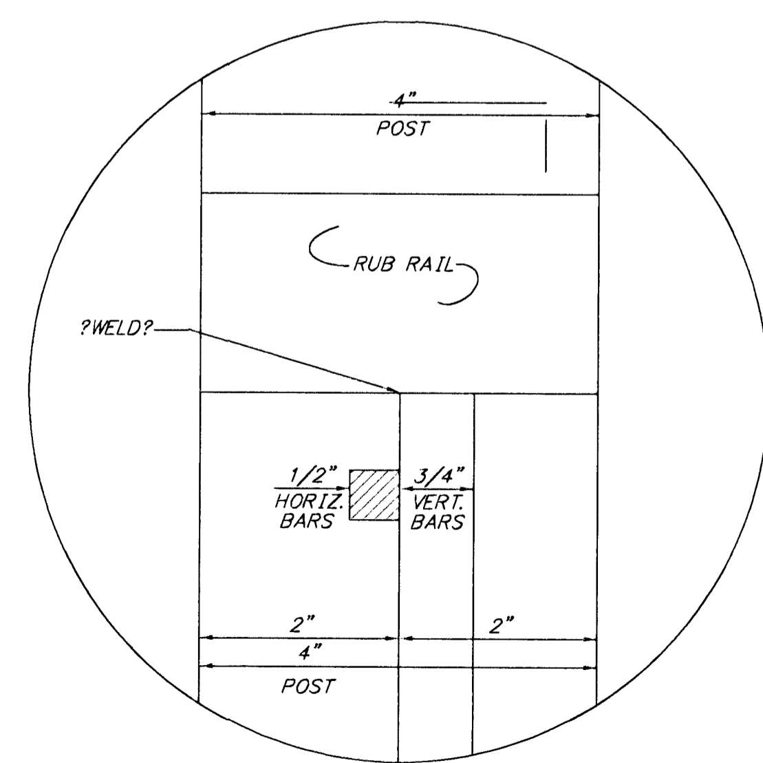
PICKET DETAIL NO SCALE
