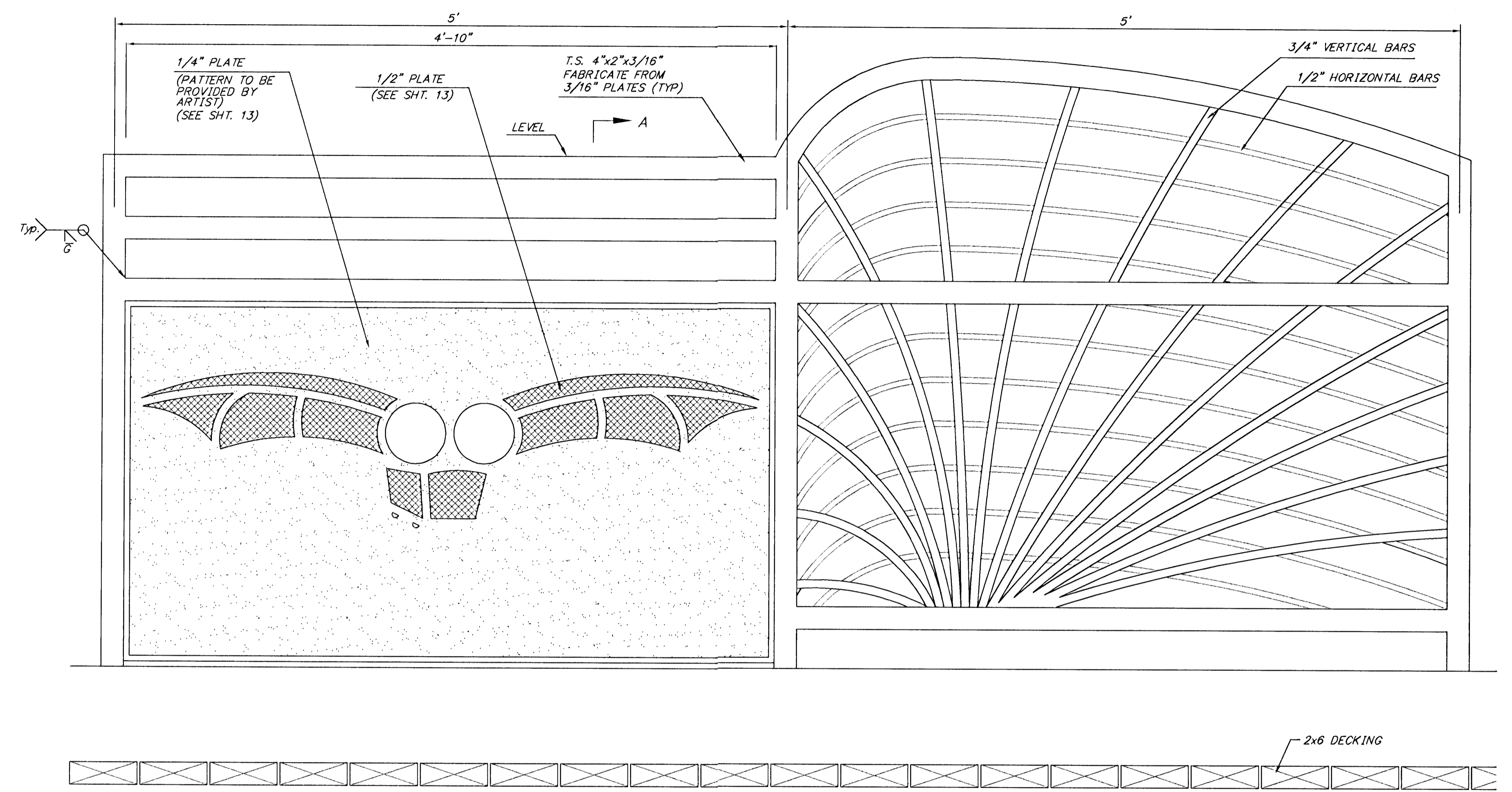
HANDRAIL ELEVATION NO SCALE
