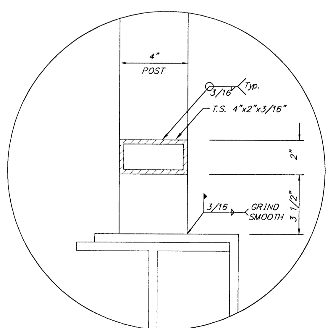
BOTTOM HANDRAIL DETAIL NO SCALE
