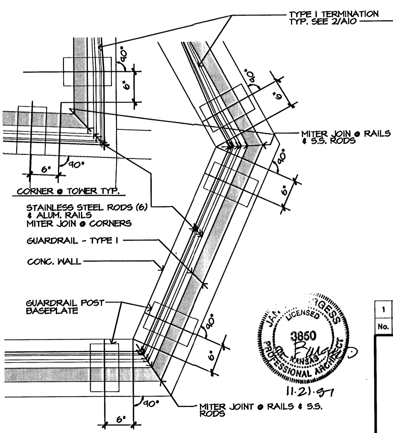
D ENLARGED CORNER PLAN GUARDRAIL TYPE I NORTHEAST LOCATION 0' 6' 1' 1"=1'-0"
