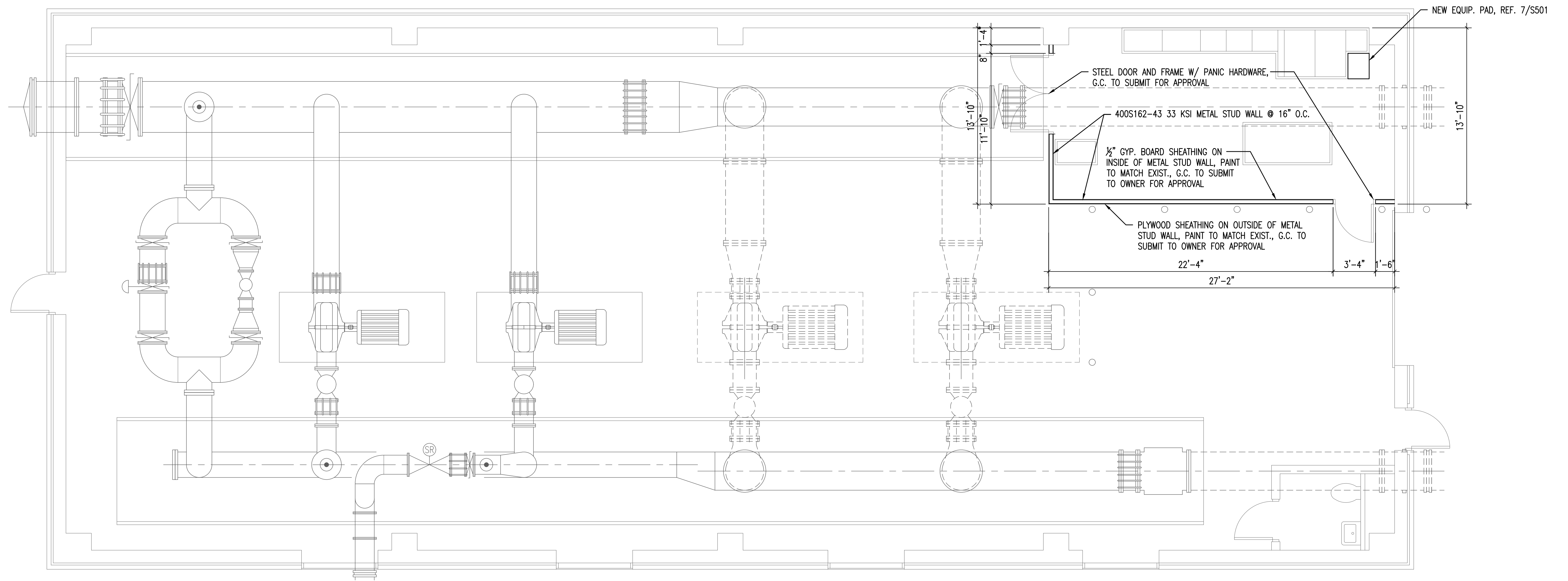
A WALL FRAMING PLAN 0' 2' 4' 6' 10' SCALE: 1/4" = 1'-0"
