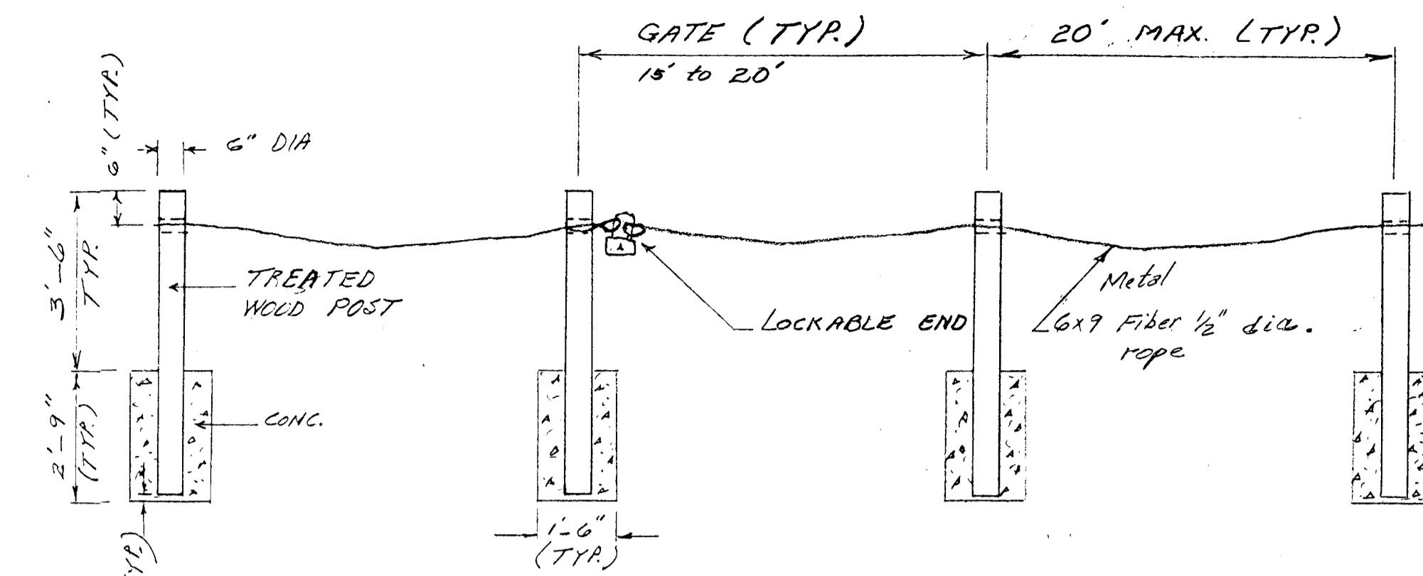
POST & CABLE DETAIL
